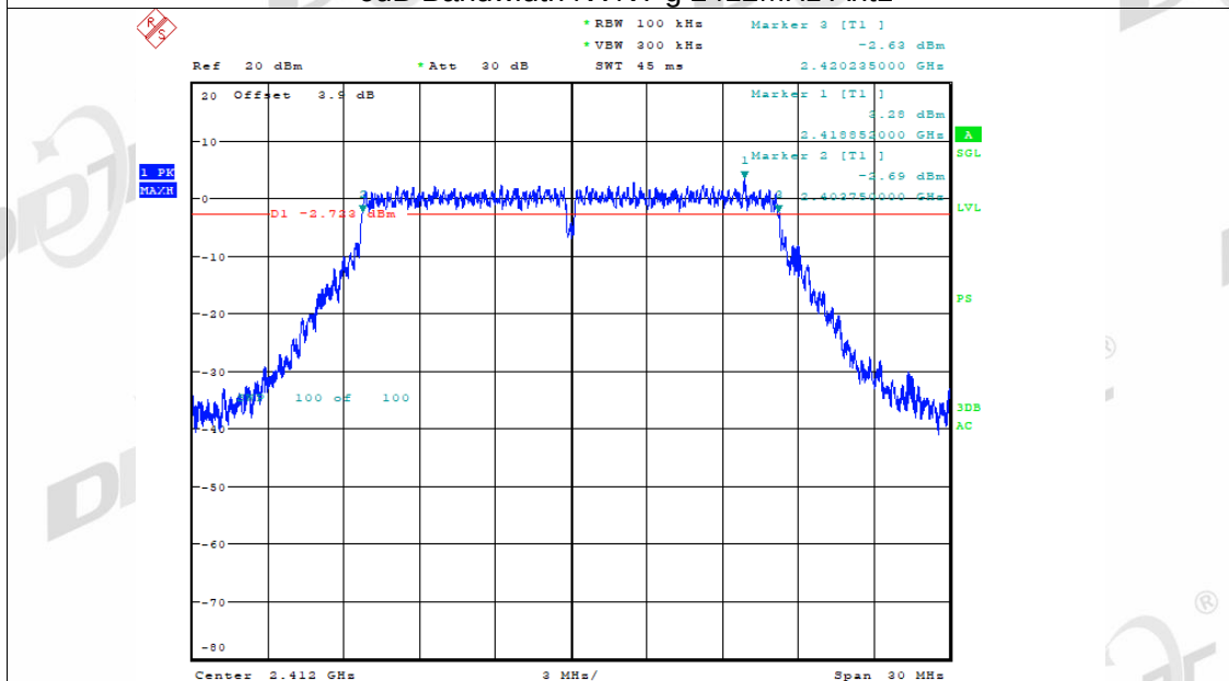
-6dB Bandwidth NVNT g 2412MHz Ant1
