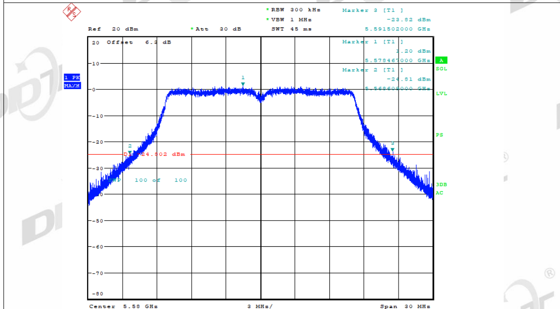
-26dB Bandwidth NVNT a 5580MHz Ant1
