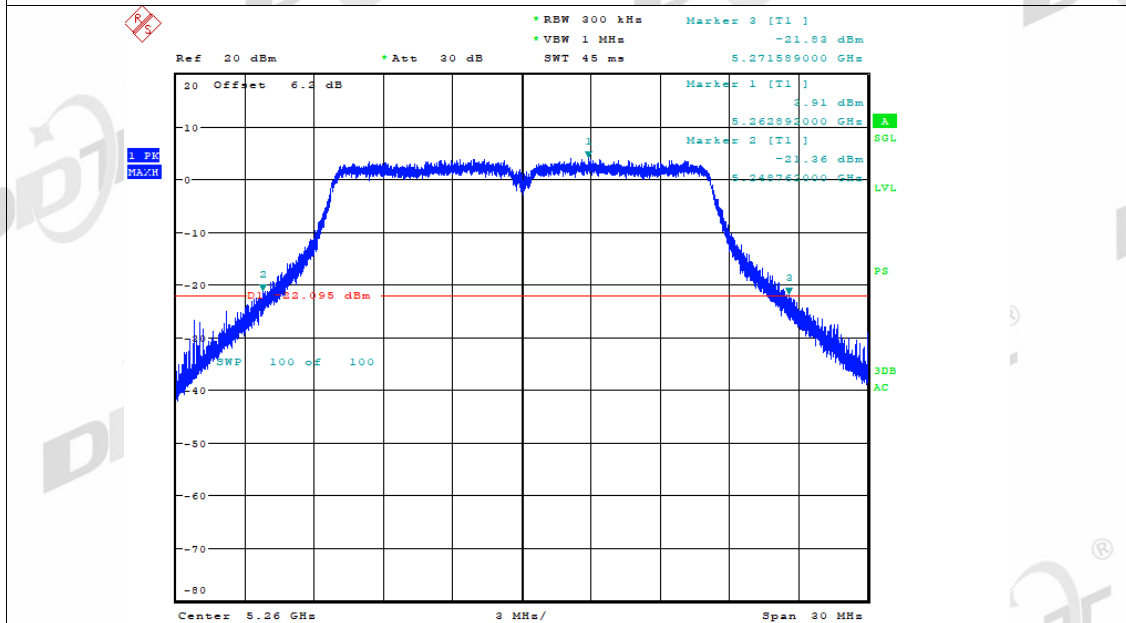
-26dB Bandwidth NVNT a 5260MHz Ant1
