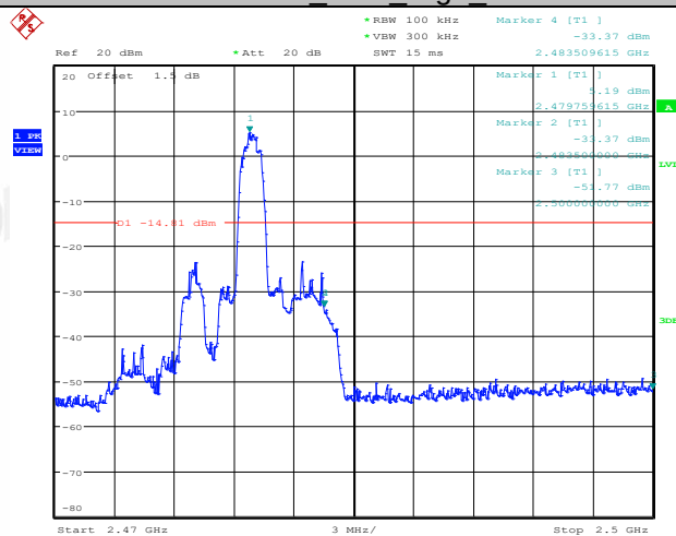
3DH5_Ant1_High_2480
