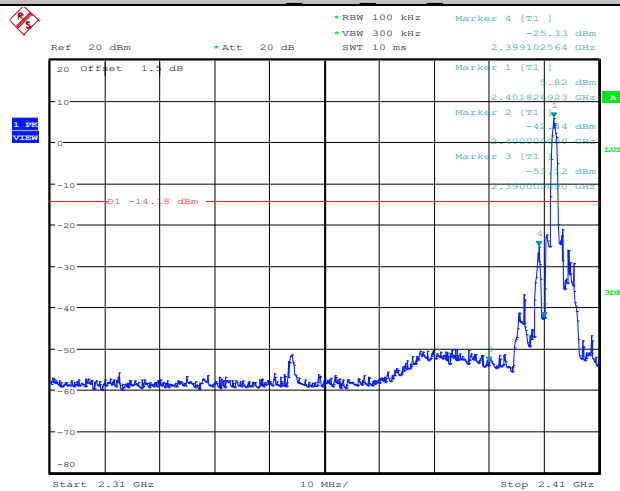
3DH5_Ant1_Low_2402
