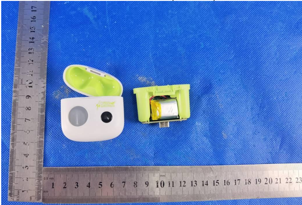
OPEN VIEW OF EUT(FIGURE 1)
