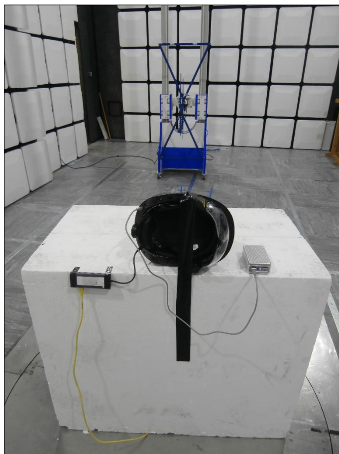
Figure 22 - Test Setup - 30 MHz to 1 GHz - Z Orientation
