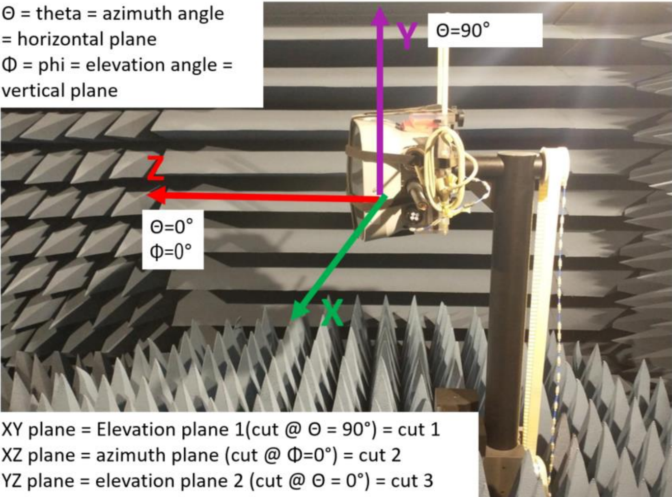
85 86 Figure 2: Wifi measurement axis setup 87
