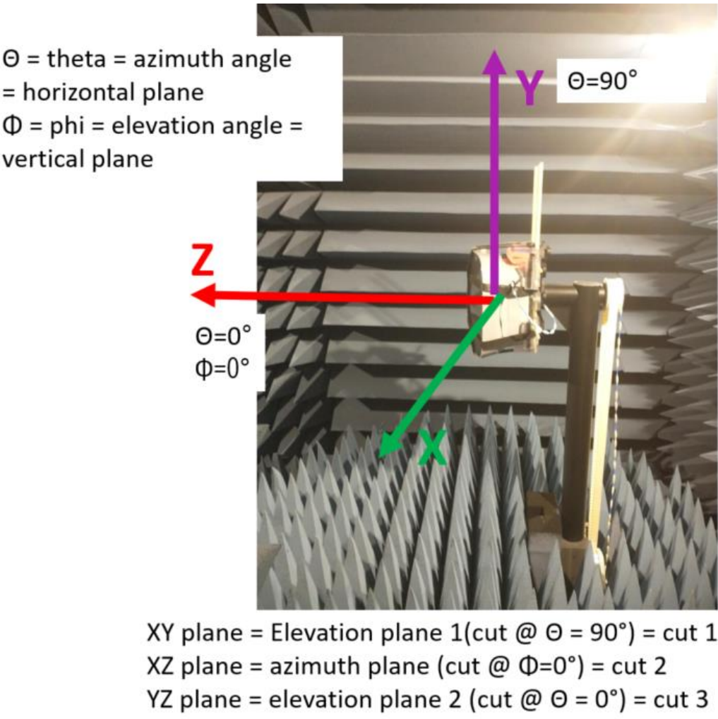
Figure 3: LTE/GNSS measurement axis setup
