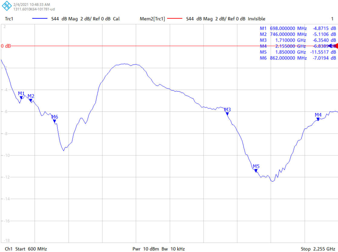
129 130 Figure 6: Return loss measurement result
