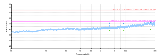
Figure 8.6-7: Radiated spurious emissions on Mid channel
