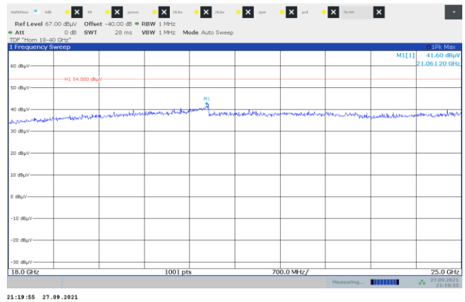
Figure 8.6-13: Radiated spurious emissions on Mid channel
