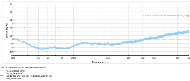
Figure 8.6-6: Radiated spurious emissions on Low channel
