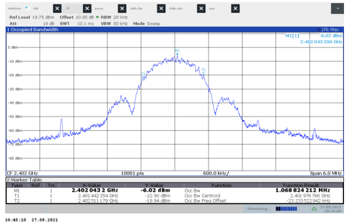
Figure 8.4-4: 99% occupied bandwidth Low channel
