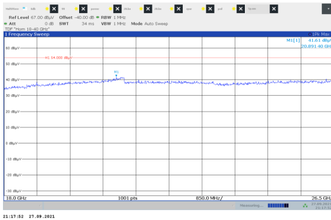
Figure 8.6-12: Radiated spurious emissions on Low channel
