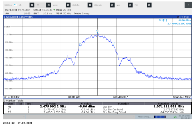
Figure 8.4-6: 99% occupied bandwidth High channel
