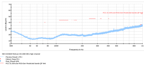
Figure 8.6-8: Radiated spurious emissions on High channel
