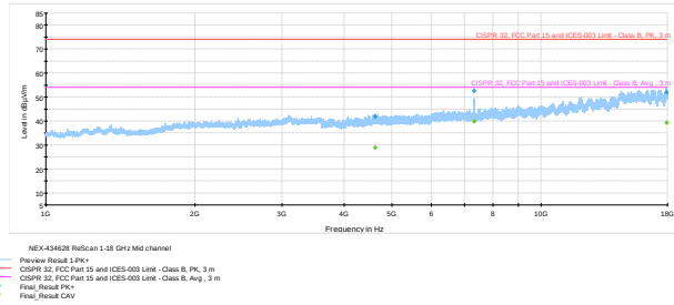
Figure 8.6-10: Radiated spurious emissions on Mid channel
