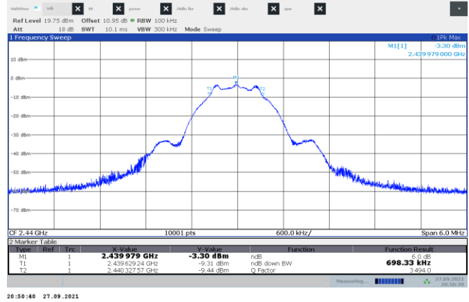
Figure 8.4-2: 6 dB bandwidth Mid channel
