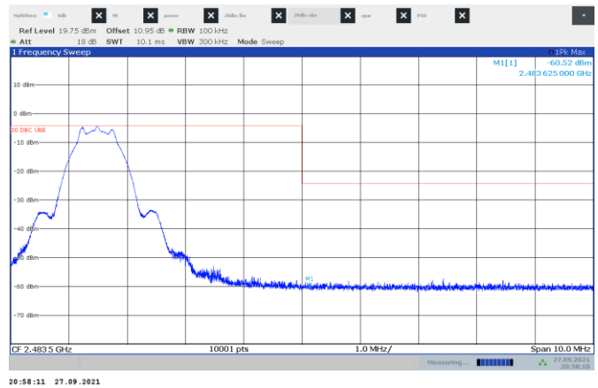
Figure 8.6-2: Band edge spurious emissions at 2483.5 MHz
