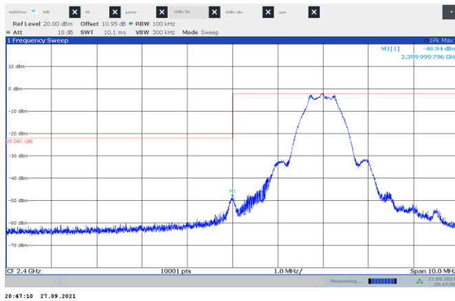
Figure 8.6-1: Band edge spurious emissions at 2400 MHz
