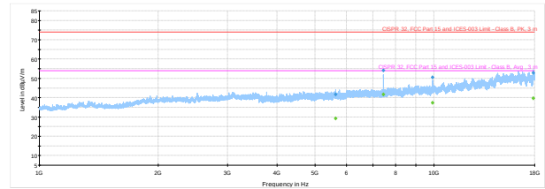
Figure 8.6-9: Radiated spurious emissions on Low channel
