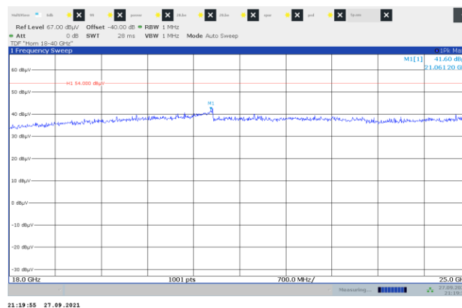
Figure 8.6-14: Radiated spurious emissions on High channel
