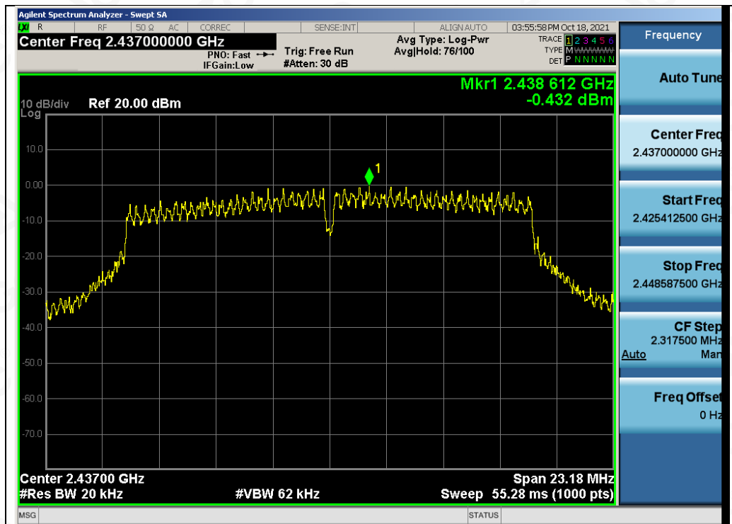
Test_Graph_802.11g_ANT1_2437_6Mbps_PSD
