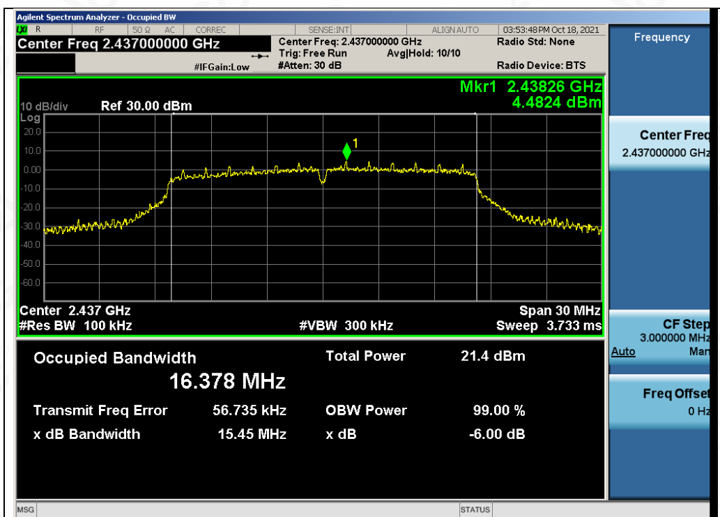
Test_Graph_802.11g_ANT1_2437_6Mbps_DTSBW
