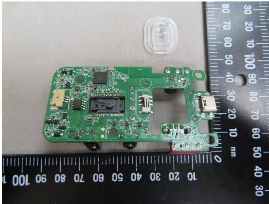
Inside View of EUT – 2
