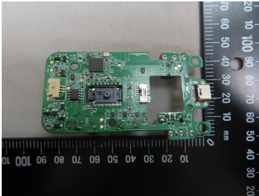
Inside View of EUT – 4
