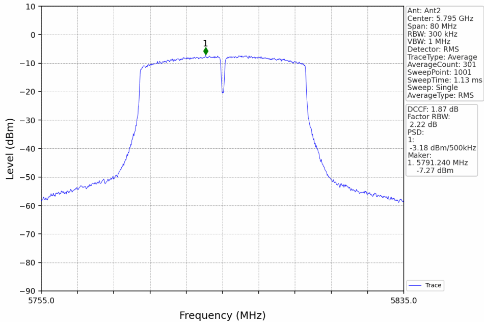
802.11ac(VHT40)_HCH_5795MHz_MIMO_NTNV
