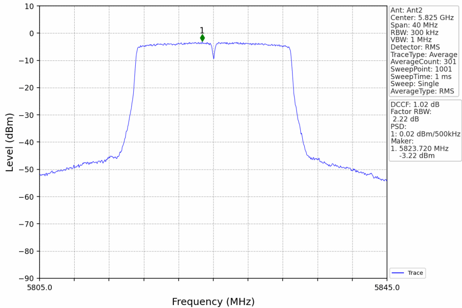
802.11ac(VHT20)_HCH_5825MHz_MIMO_NTNV
