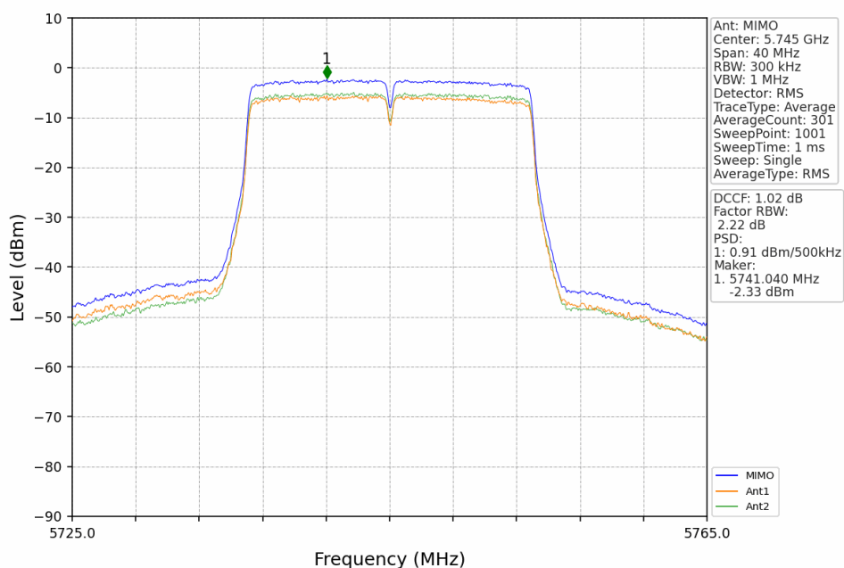
802.11ac(VHT20)_LCH_5745MHz_MIMO_NTNV
