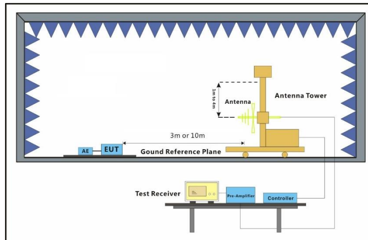
Above 1GHz
