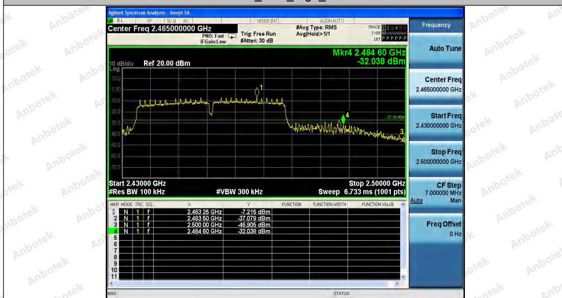
11N40_Ant1_High_2452
