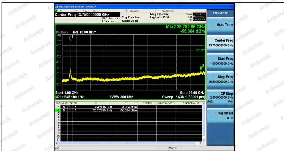
11G_Ant2_2462_0~Reference
