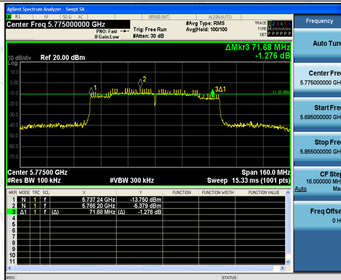
11AC80SISO_Ant2_5775
