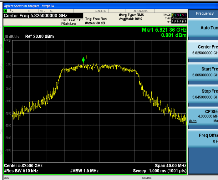
11AC20SISO_Ant2_5825
