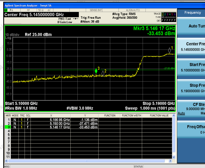
11AC80SISO_Ant1_High_5210
