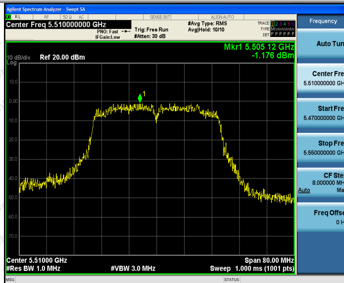
11AC40SISO_Ant2_5510
