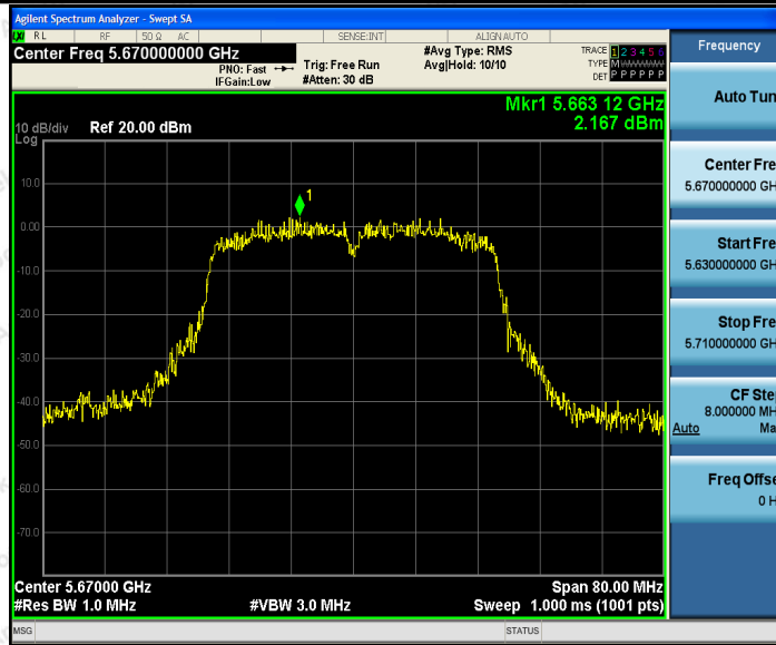
11AC40SISO_Ant2_5670
