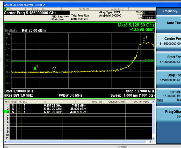
11N20SISO_Ant2_Low_5260
