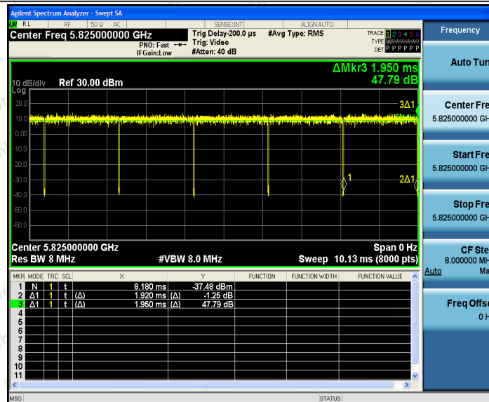
11AC20SISO_Ant2_5825
