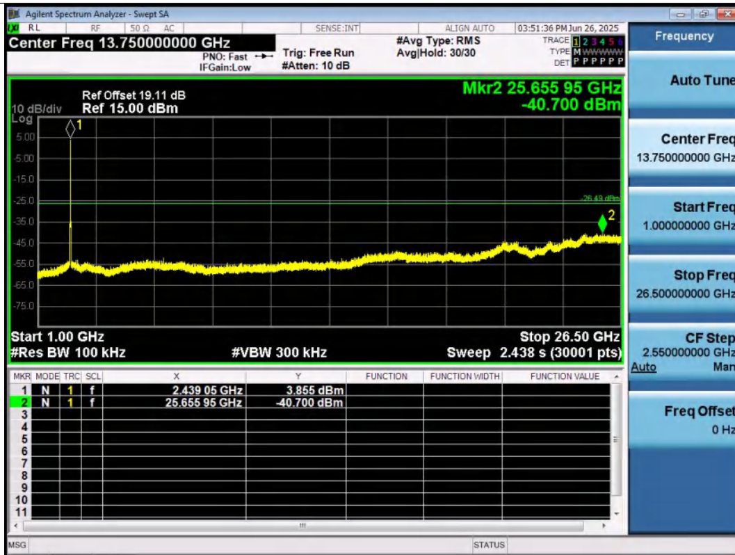
11G-Ant1-2437-1000~26500-PASS
