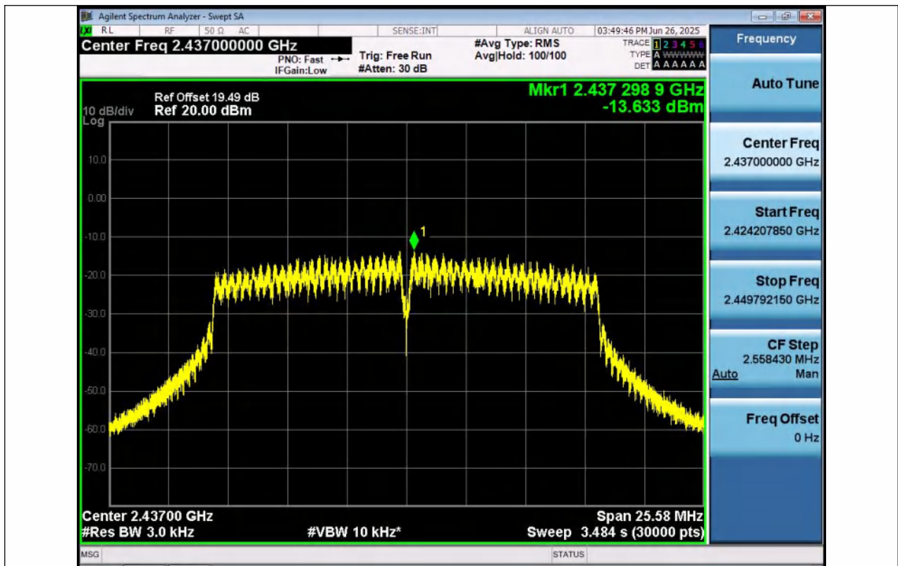
11G-Ant1-2437-PASS
