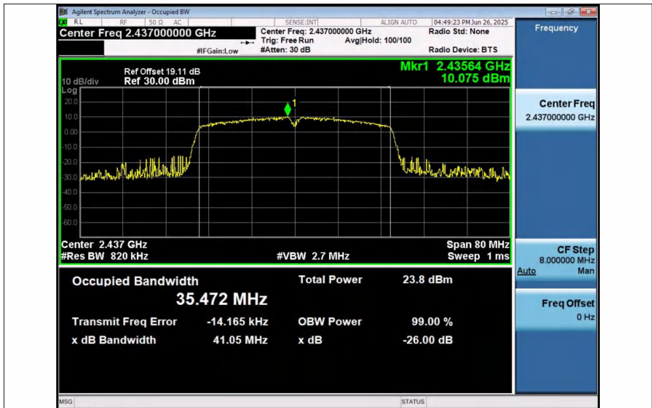
11N40SISO-Ant1-2437
