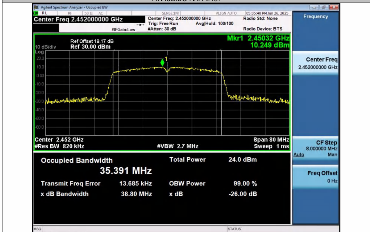
11N40SISO-Ant1-2452
