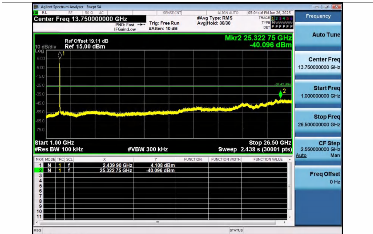
11N40SISO-Ant1-2437-1000~26500-PASS
