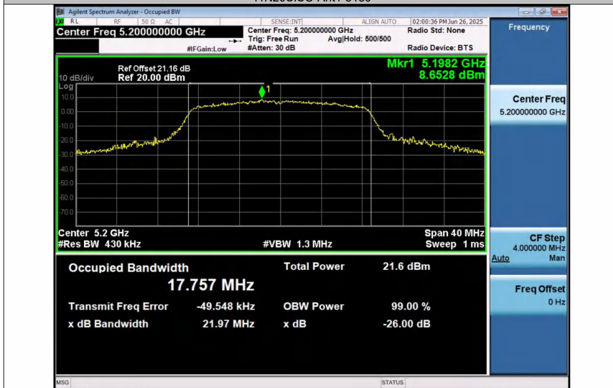
11N20SISO-Ant1-5200
