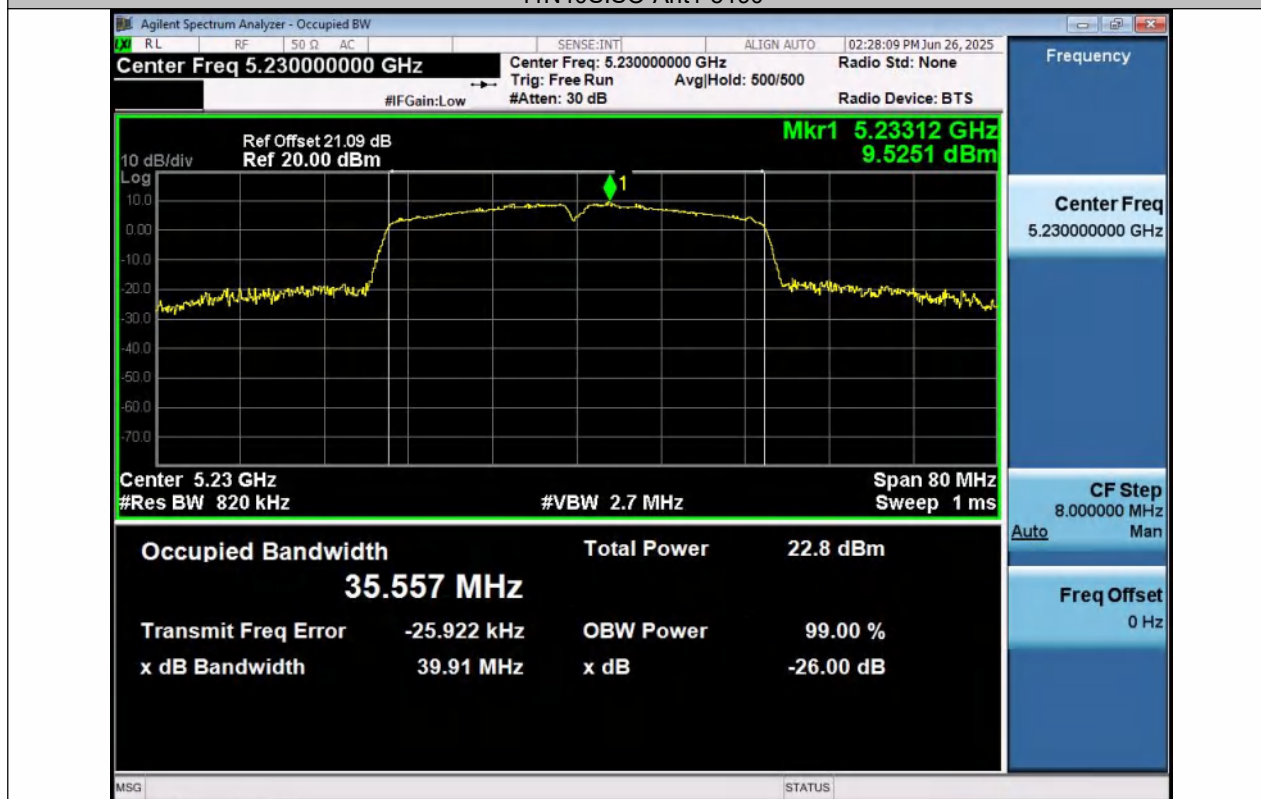
11N40SISO-Ant1-5230
