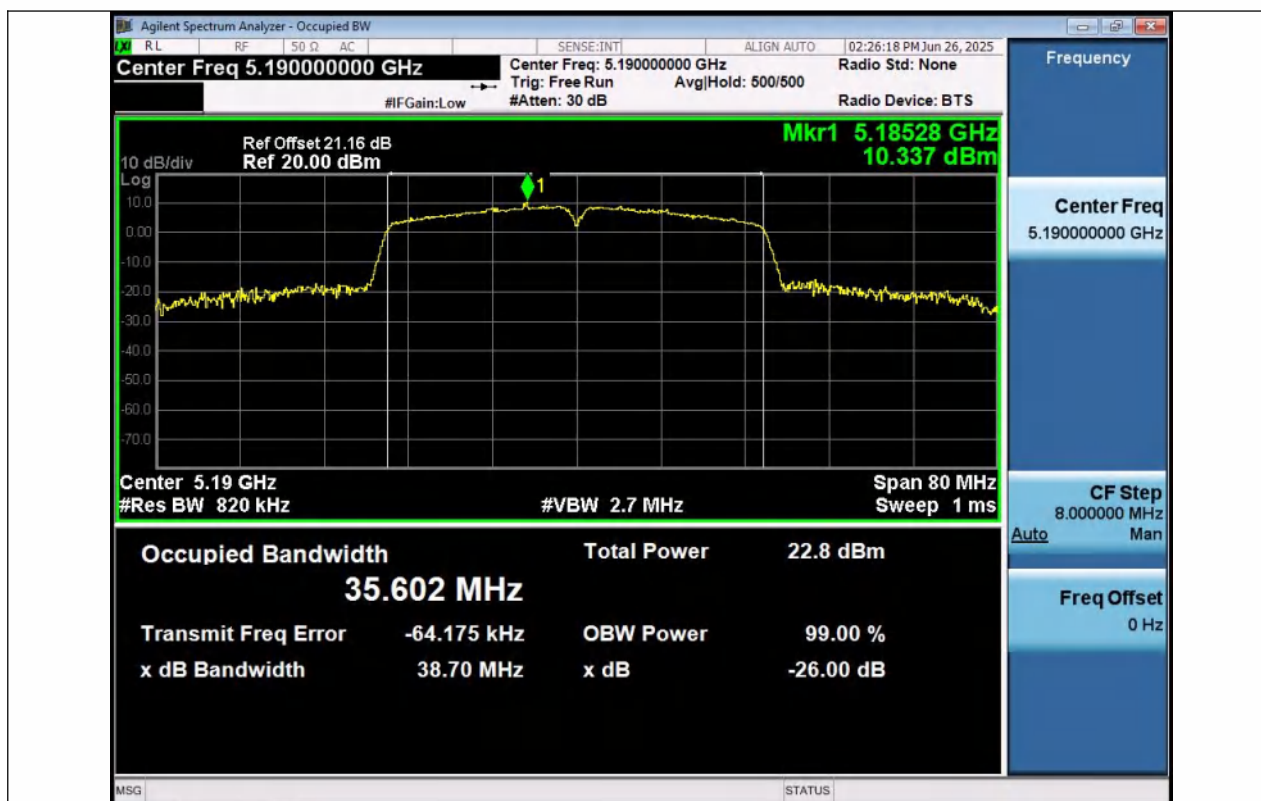
11N40SISO-Ant1-5190
