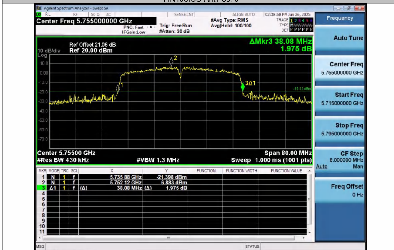
11N40SISO-Ant1-5755
