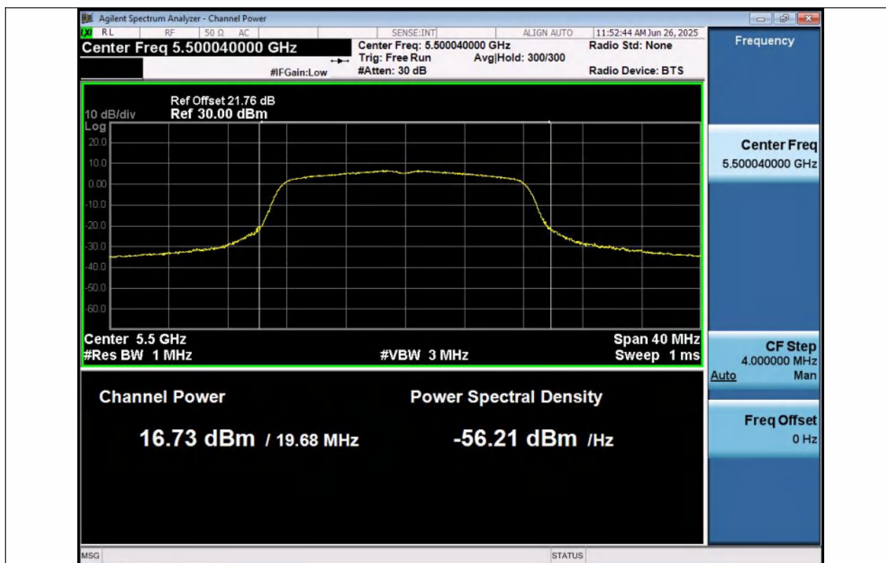
11A-Ant1-5500-PASS
