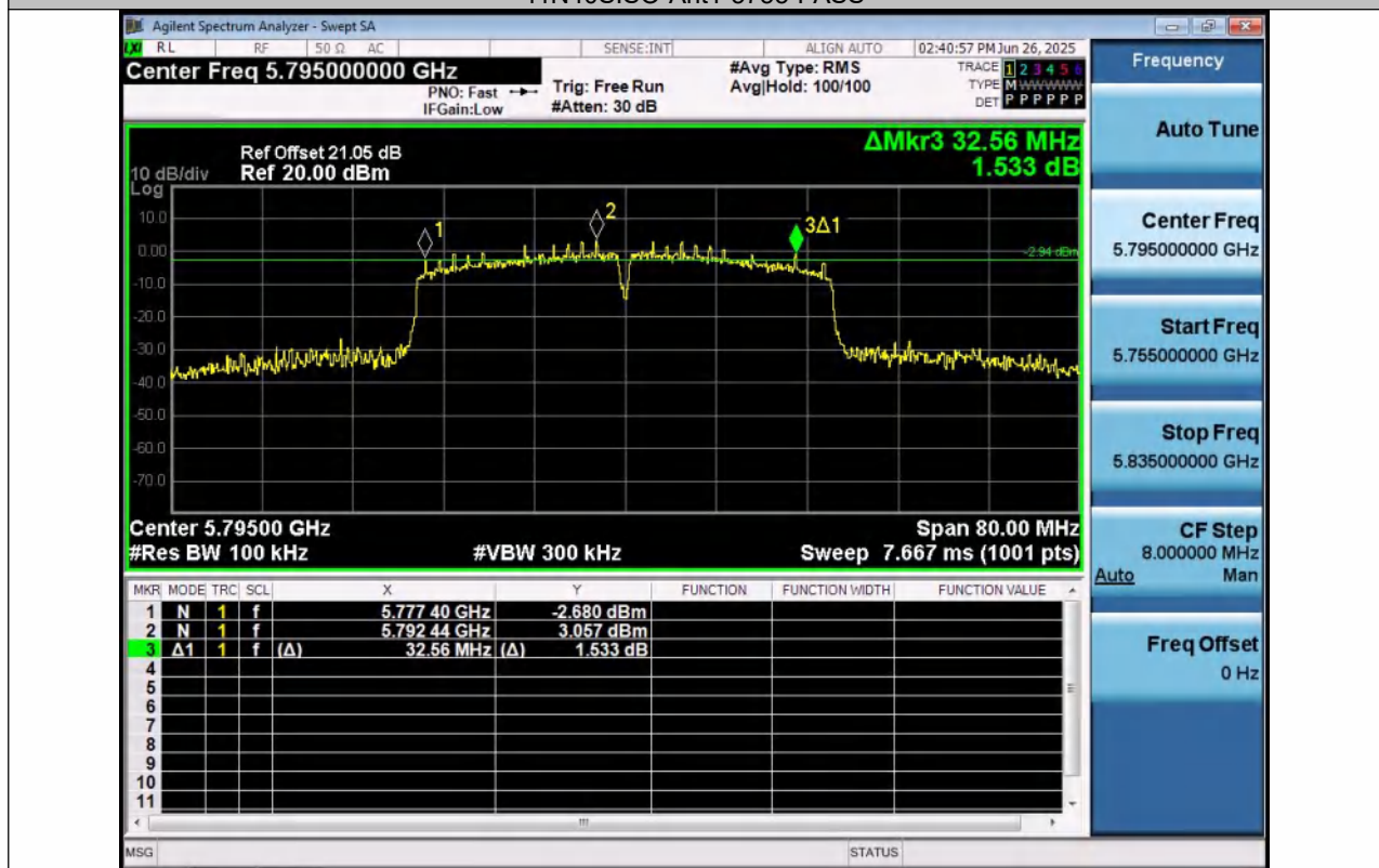
11N40SISO-Ant1-5795-PASS
