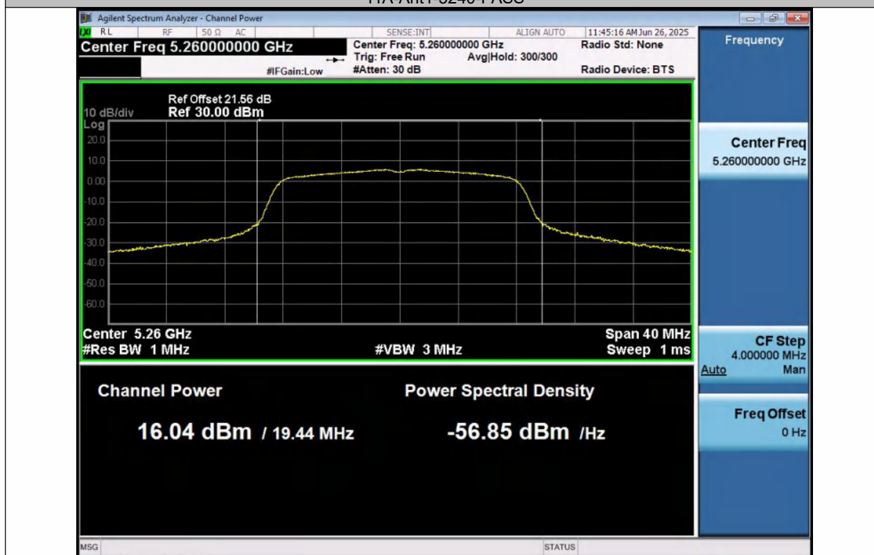
11A-Ant1-5260-PASS
