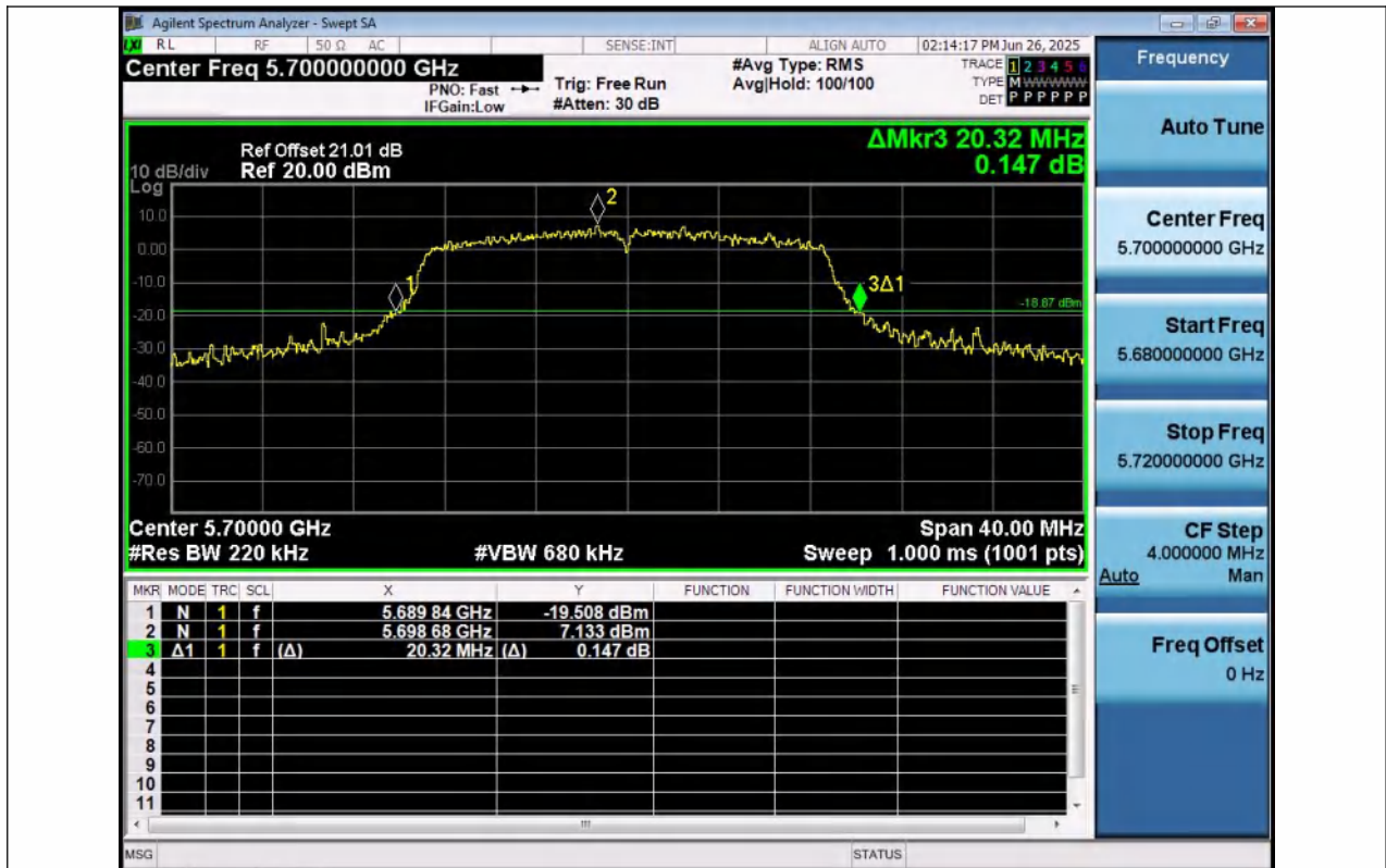
11N20SISO-Ant1-5700
