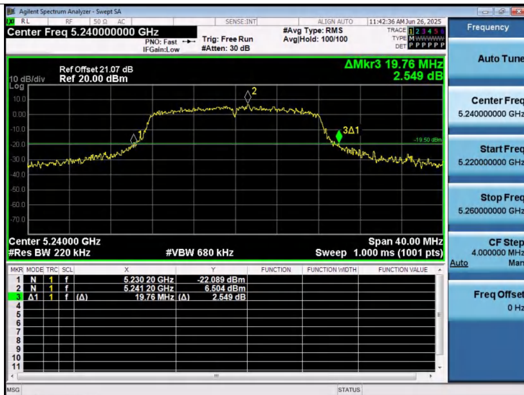
11A-Ant1-5240
