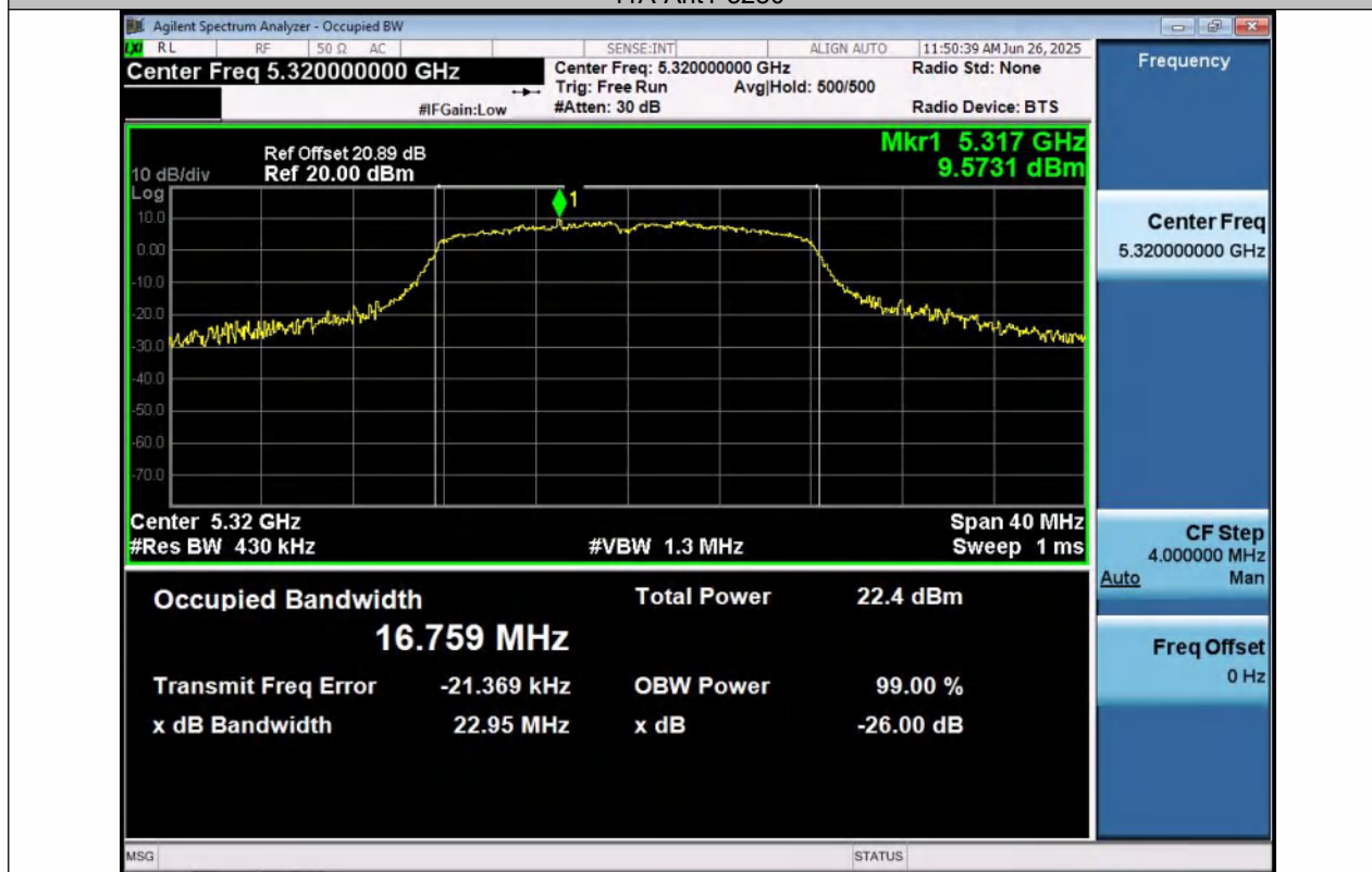
11A-Ant1-5320
