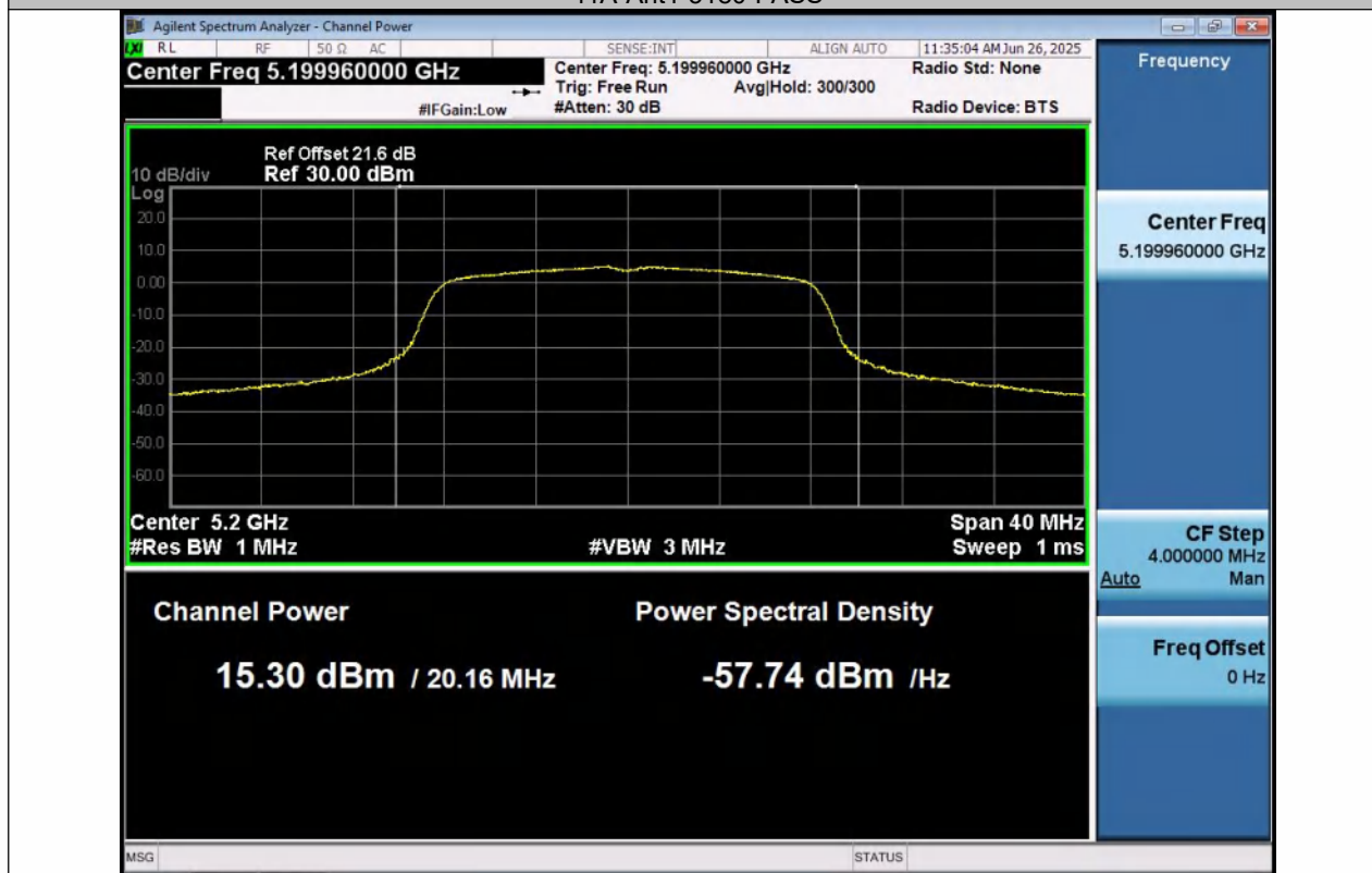
11A-Ant1-5200-PASS
