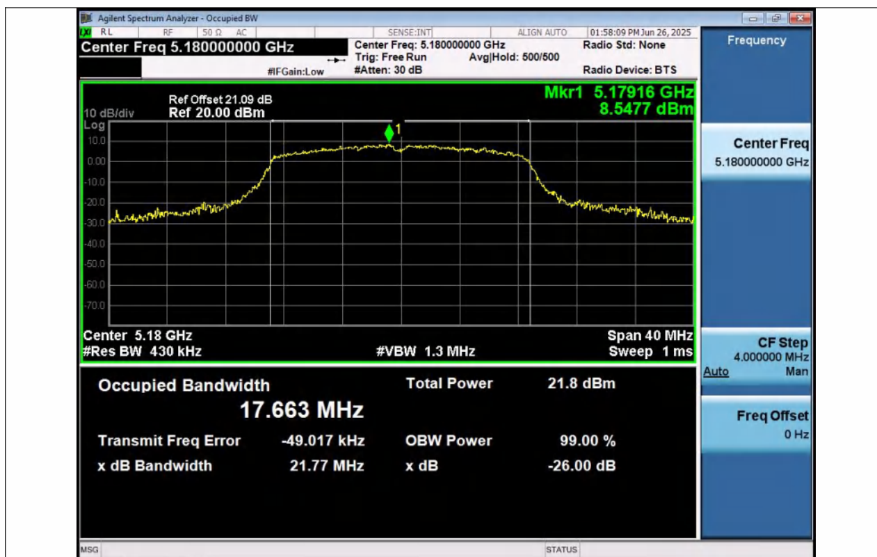
11N20SISO-Ant1-5180
