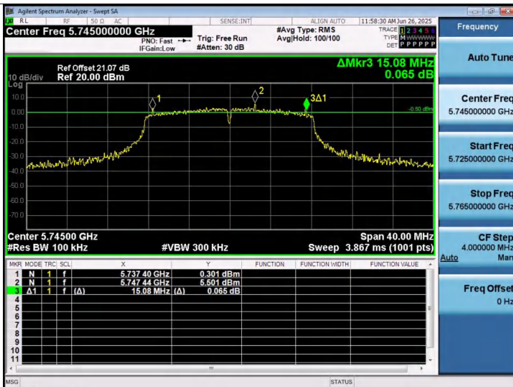
11A-Ant1-5745-PASS
