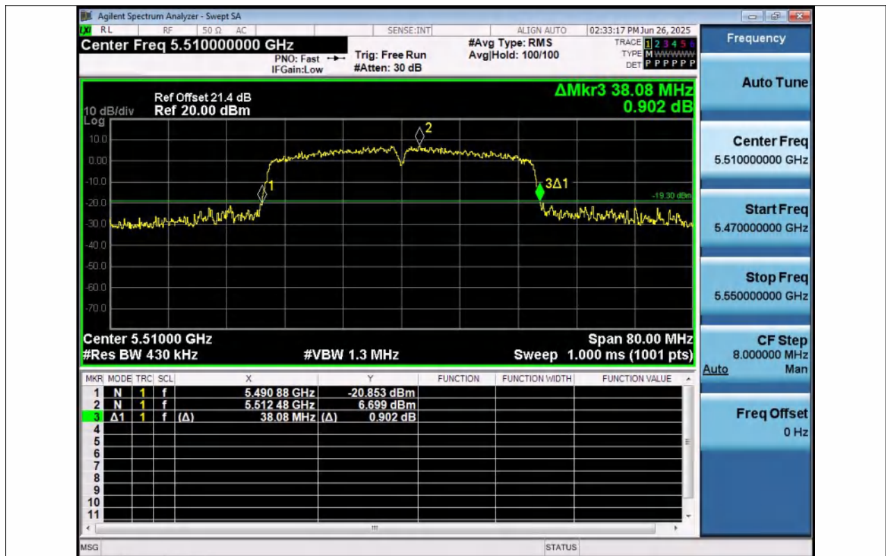
11N40SISO-Ant1-5510
