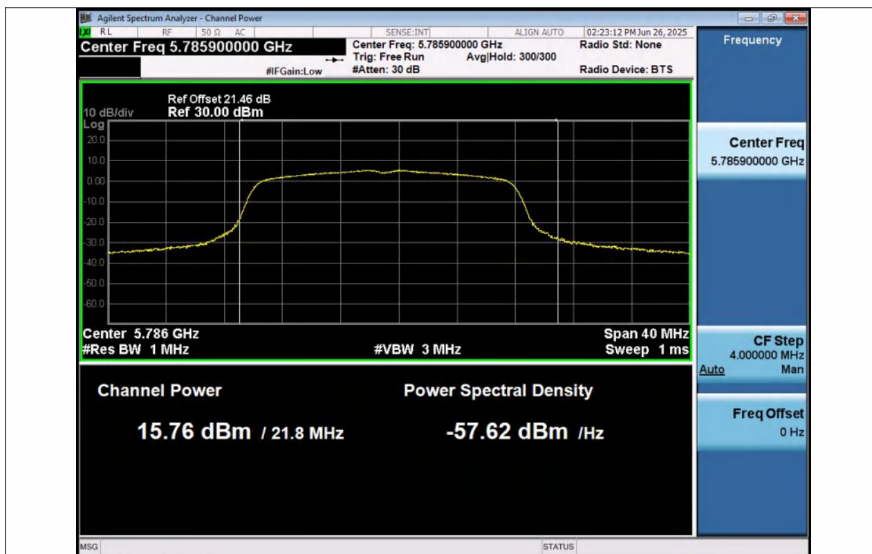
11N20SISO-Ant1-5785-PASS
