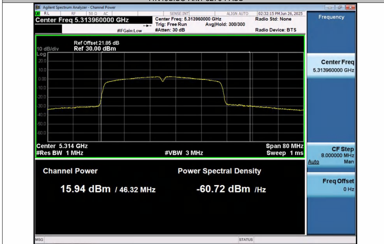
11N40SISO-Ant1-5310-PASS
