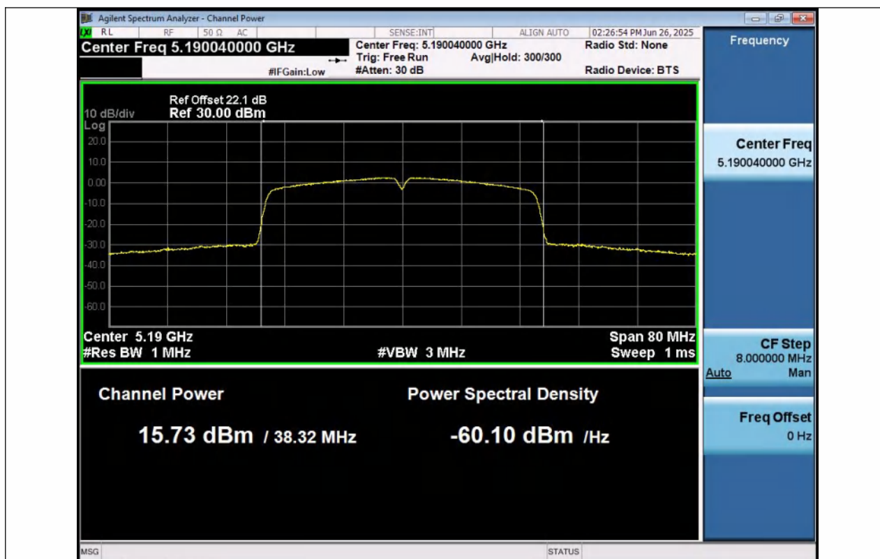
11N40SISO-Ant1-5190-PASS
