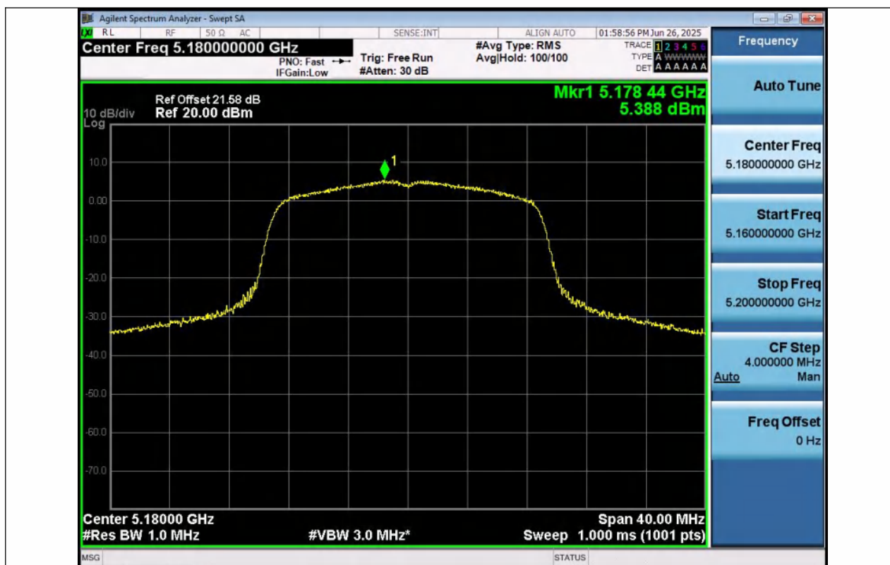
11N20SISO-Ant1-5180-PASS
