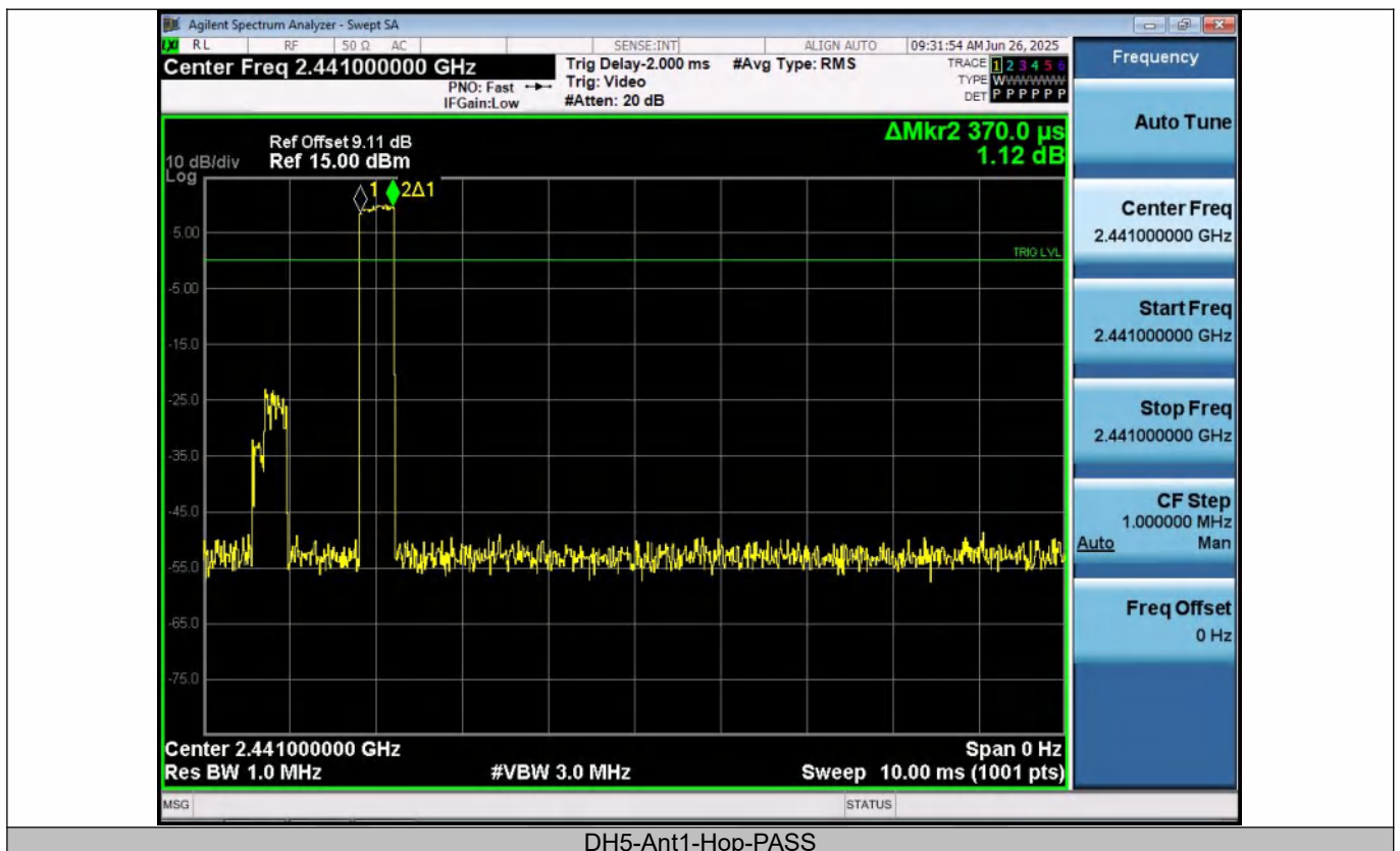
DH5-Ant1-Hop-PASS
