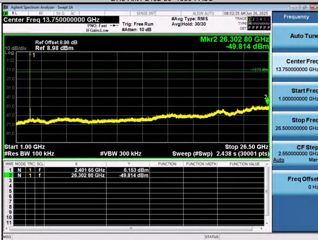
DH5-Ant1-2402-1000~26500-PASS
