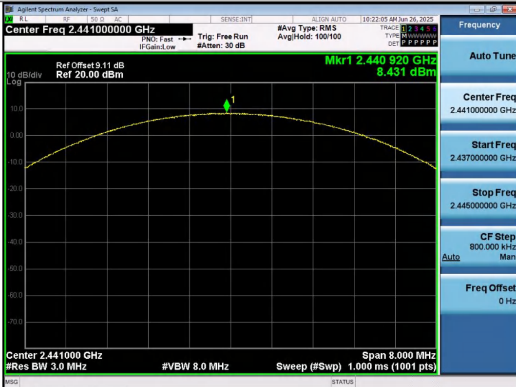
3DH5-Ant1-2441-PASS
