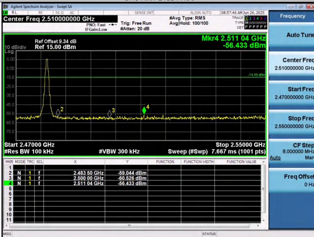
DH5-Ant1-2480-PASS
