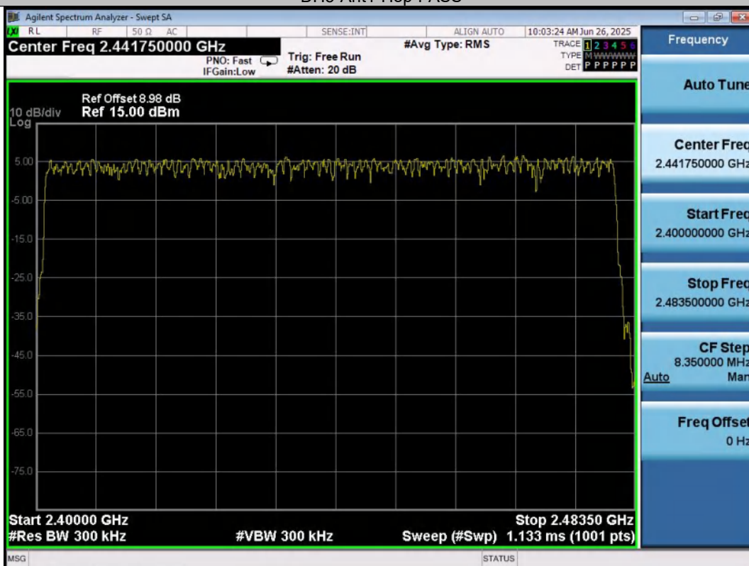
2DH5-Ant1-Hop-PASS
