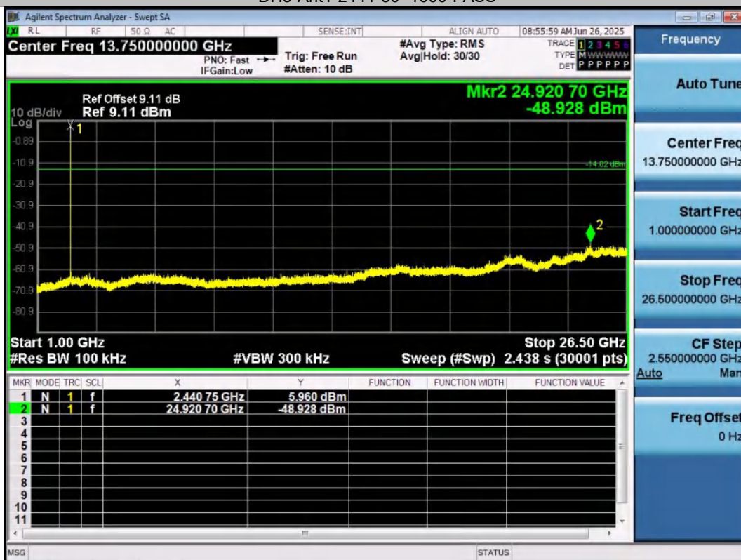
DH5-Ant1-2441-1000~26500-PASS
