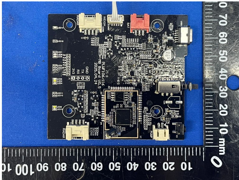
PCB 2
