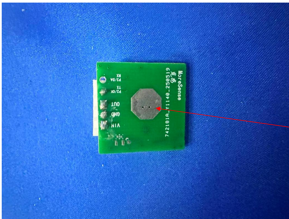
10G Radar ANT
