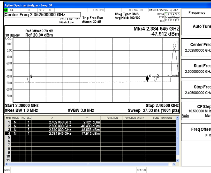
BLE_1M_Ant2_Low_2402_Peak
