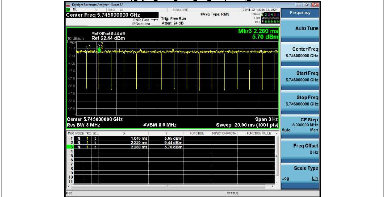
Duty_Cycle_NVNT_ANT1_802_11ac(VHT20)_5745
