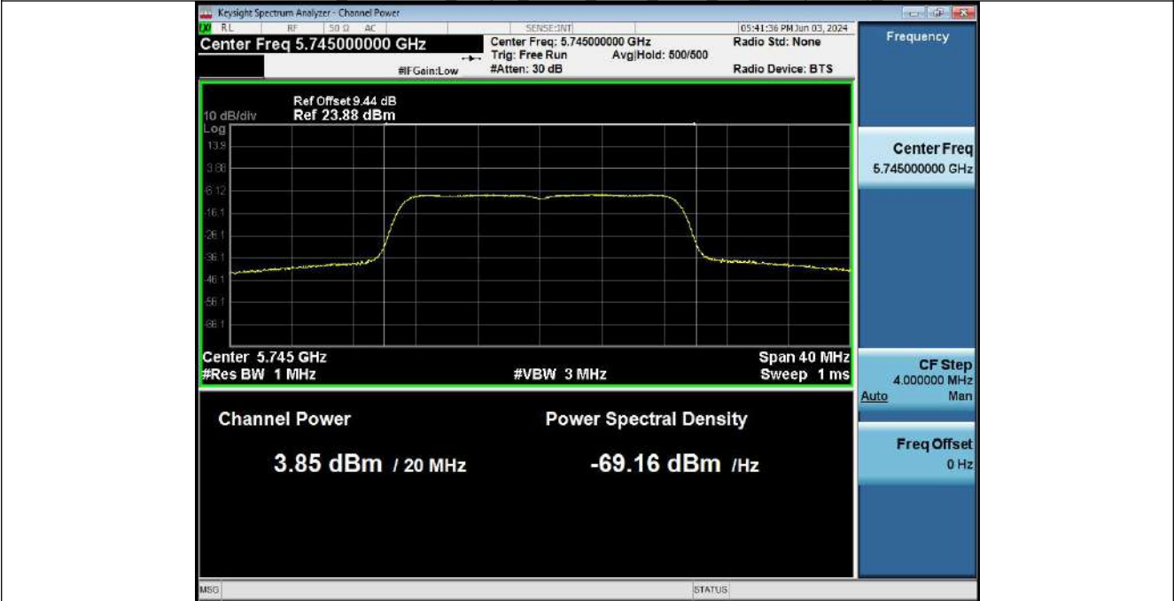
Maximum_Conducted_Output_Power_NVNT_ANT1_802_11ac(VHT20)_5745
