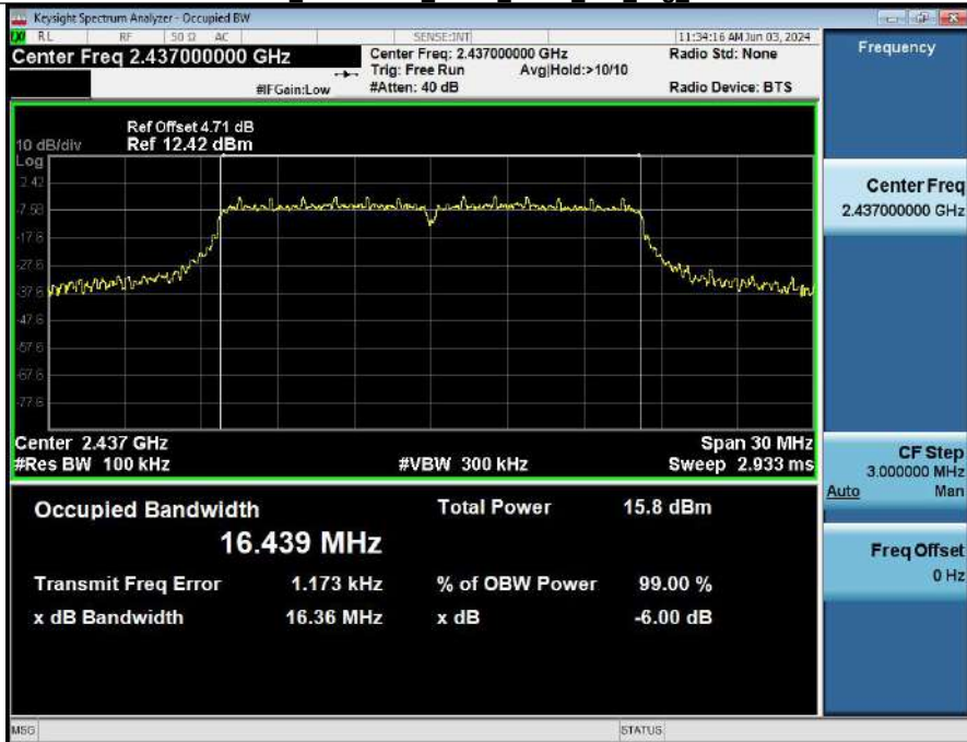
-6dB_Bandwidth_NVNT_ANT1_802_11g_2437
