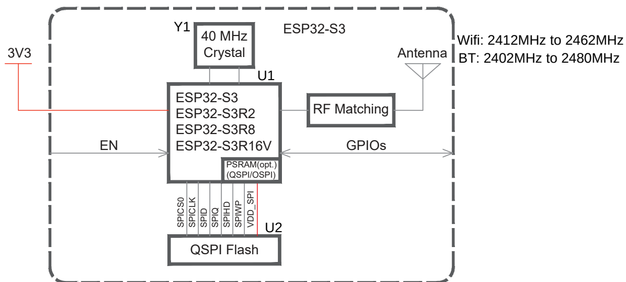
Figure 1: ESP32-S3 Block Diagram
