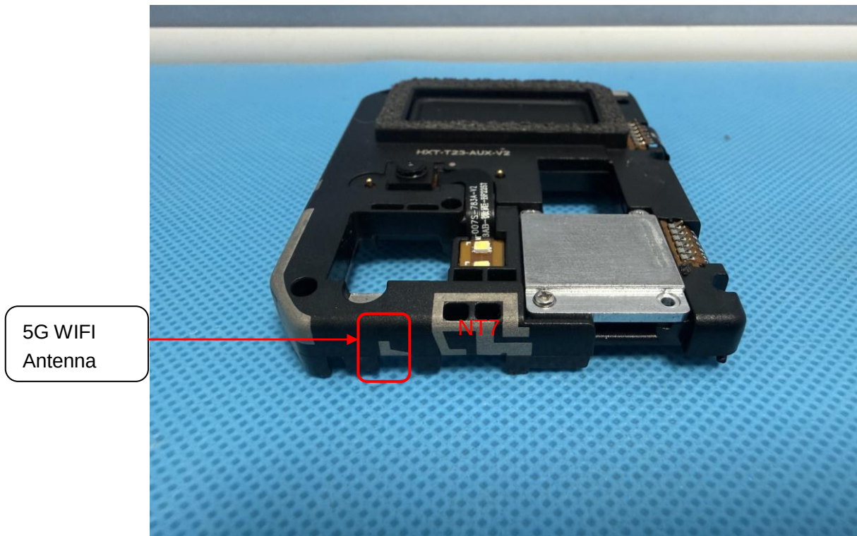
Antenna View of EUT (Figure 6)
