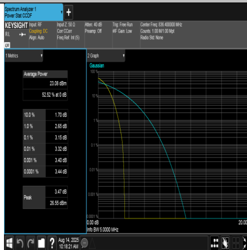
Band5-4182-1-PASS
