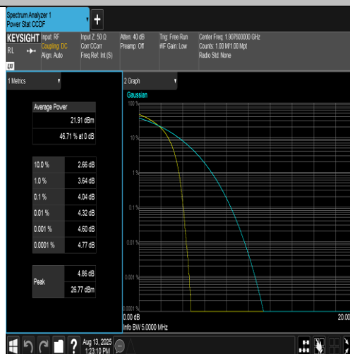
Band2-9538-5-PASS
