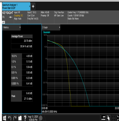
Band4-1312-2-PASS
