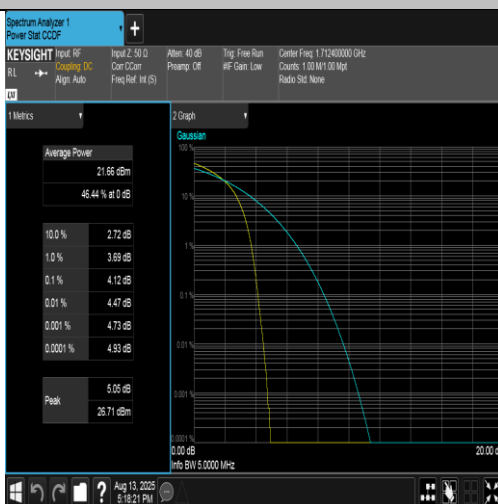
Band4-1312-5-PASS
