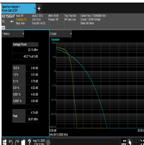
Band4-1413-3-PASS
