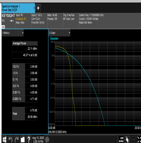
Band4-1413-4-PASS
