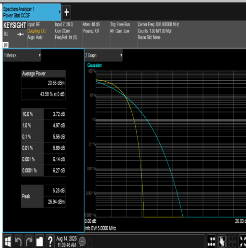
Band5-4182-4-PASS
