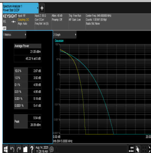
Band5-4233-1-PASS
