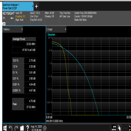
Band5-4182-2-PASS
