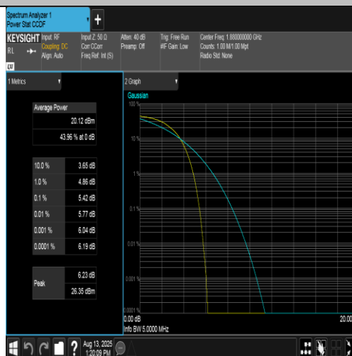
Band2-9400-4-PASS
