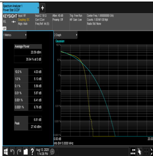
Band2-9400-2-PASS
