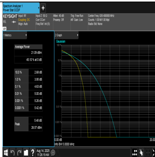
Band5-4132-1-PASS
