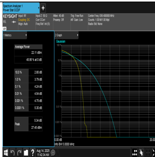
Band5-4182-5-PASS
