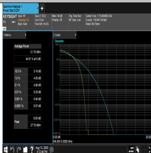
Band4-1312-3-PASS
