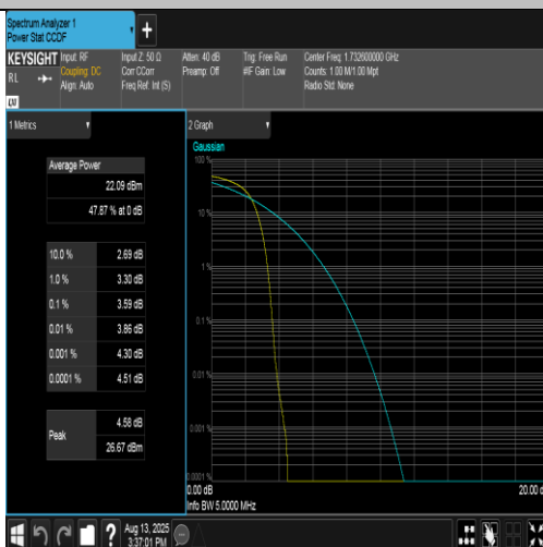
Band4-1413-2-PASS
