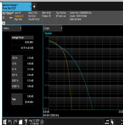
Band2-9400-3-PASS
