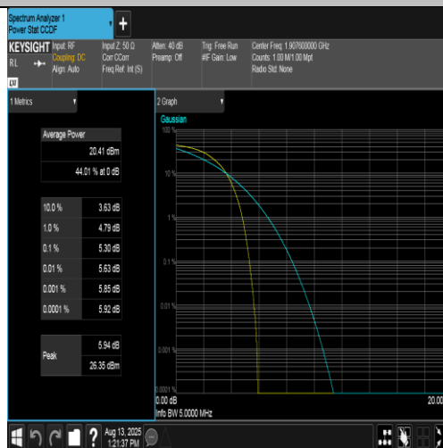
Band2-9538-4-PASS
