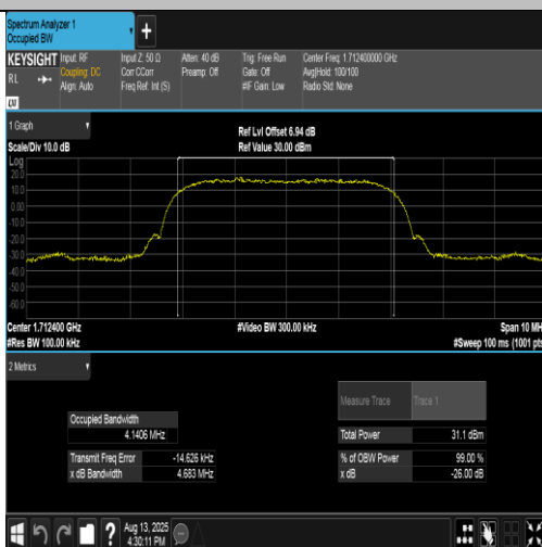
Band4-1312-2-PASS
