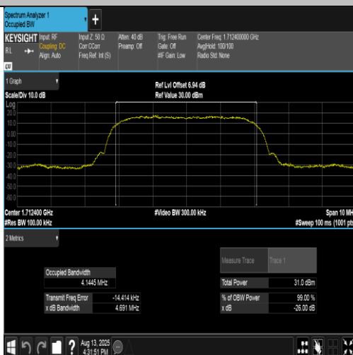
Band4-1312-3-PASS
