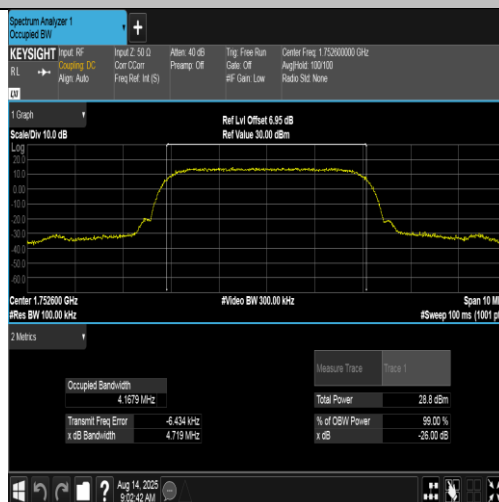
Band4-1513-2-PASS
