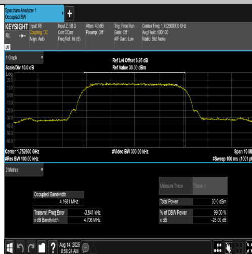
Band4-1513-1-PASS
