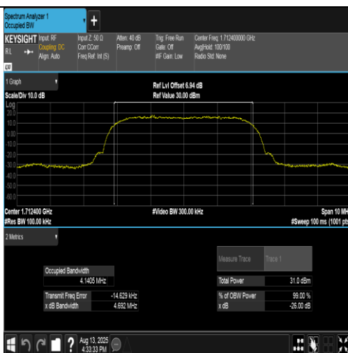
Band4-1312-4-PASS
