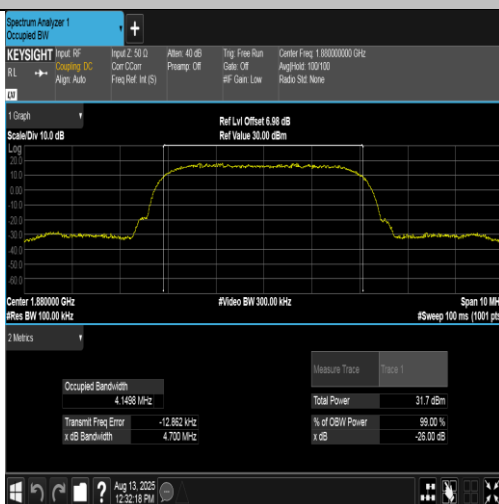
Band2-9400-1-PASS
