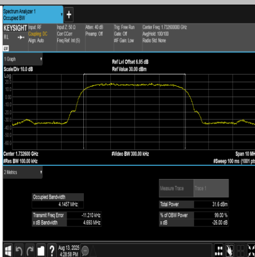
Band4-1413-1-PASS
