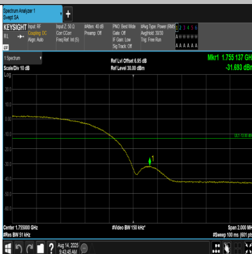
Band4-1513-3-PASS
