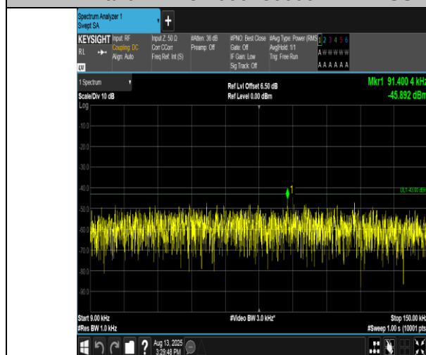
Band4-1513-0.009~0.15MHz-PASS
