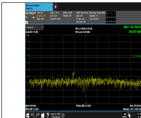
Band5-4132-0.009~0.15MHz-PASS
