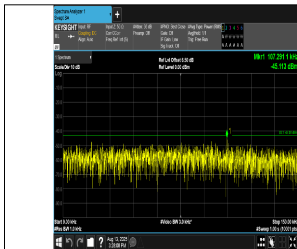
Band4-1312-0.009~0.15MHz-PASS
