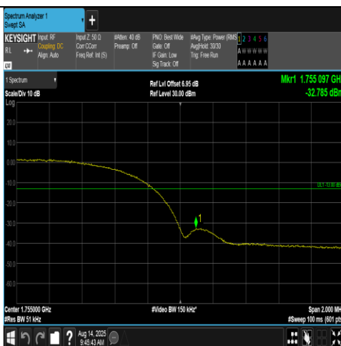
Band4-1513-4-PASS
