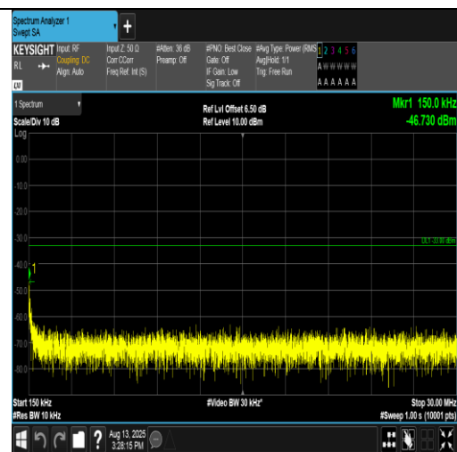
Band4-1312-0.15~30MHz-PASS
