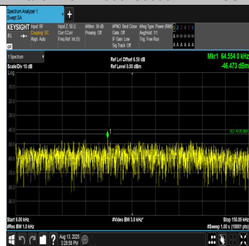
Band4-1413-0.009~0.15MHz-PASS
