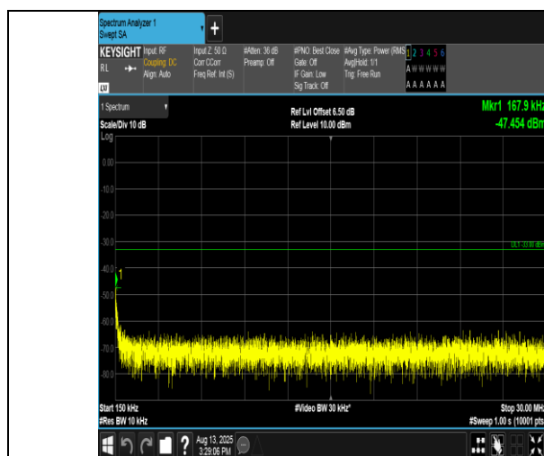
Band4-1413-0.15~30MHz-PASS
