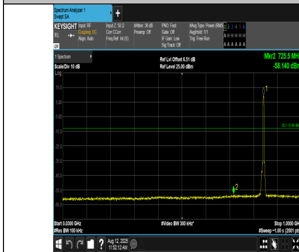
Band5-4233-30~1000MHz-PASS
