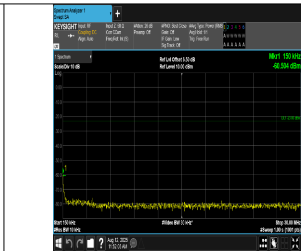
Band5-4233-0.15~30MHz-PASS
