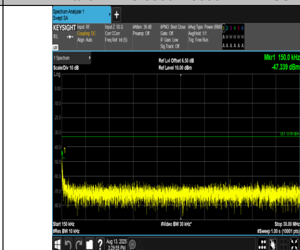
Band4-1513-0.15~30MHz-PASS
