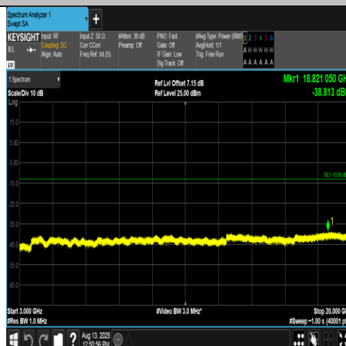
Band2-9538-4-3000~20000MHz-PASS
