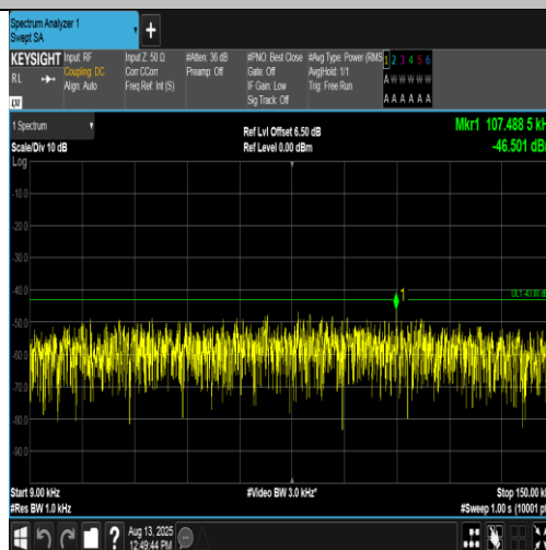
Band2-9400-4-0.009~0.15MHz-PASS
