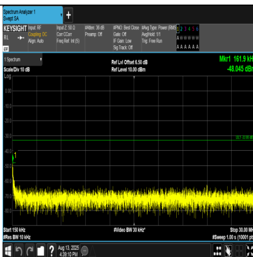
Band4-1413-1-0.15~30MHz-PASS
