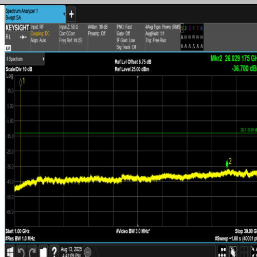
Band4-1312-2-1000~30000MHz-PASS
