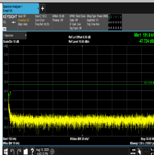
Band4-1312-3-0.15~30MHz-PASS
