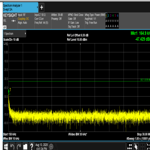
Band4-1413-2-0.15~30MHz-PASS
