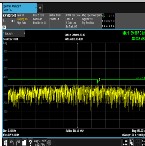
Band4-1312-2-0.009~0.15MHz-PASS
