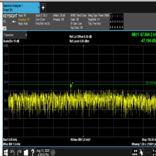
Band4-1413-1-0.009~0.15MHz-PASS
