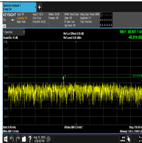
Band4-1312-1-0.009~0.15MHz-PASS
