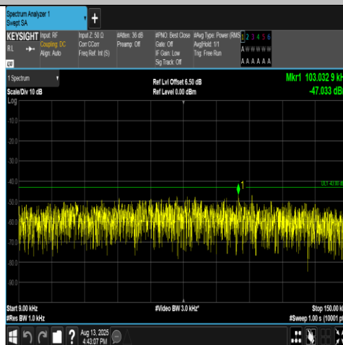
Band4-1312-3-0.009~0.15MHz-PASS
