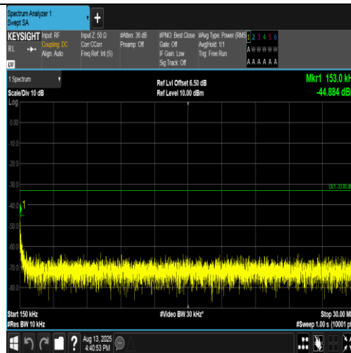
Band4-1312-2-0.15~30MHz-PASS
