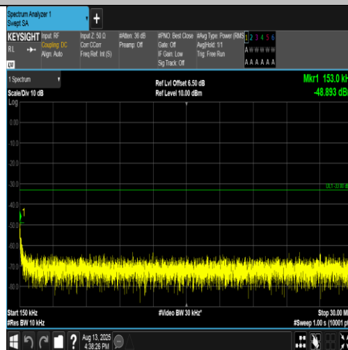
Band4-1312-1-0.15~30MHz-PASS
