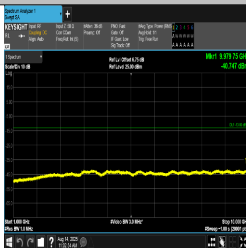
Band5-4182-4-1000~10000MHz-PASS
