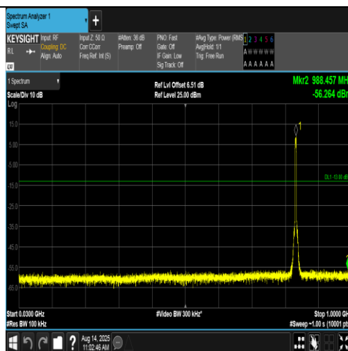
Band5-4182-4-30~1000MHz-PASS
