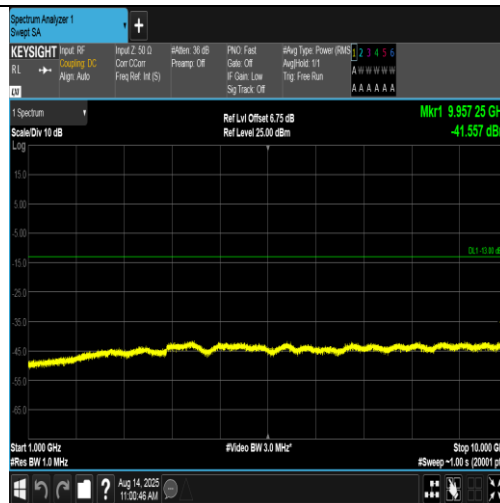
Band5-4182-3-1000~10000MHz-PASS
