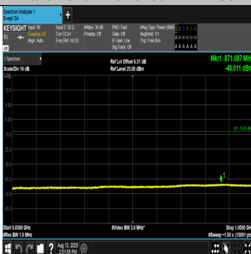
Band2-9262-1-30~1000MHz-PASS
