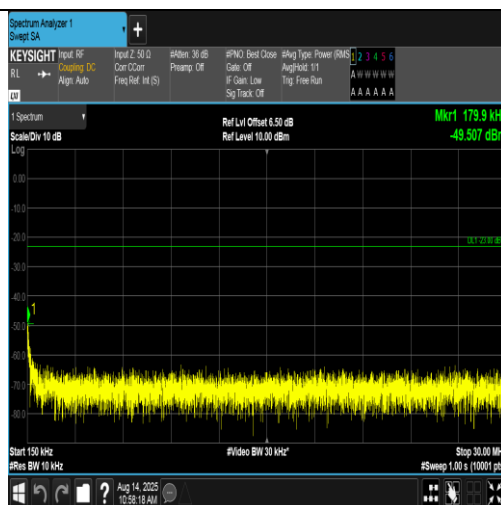
Band5-4182-2-0.15~30MHz-PASS
