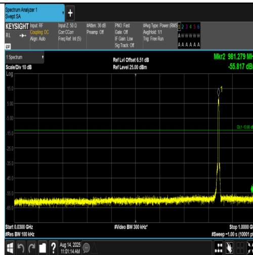
Band5-4233-3-30~1000MHz-PASS
