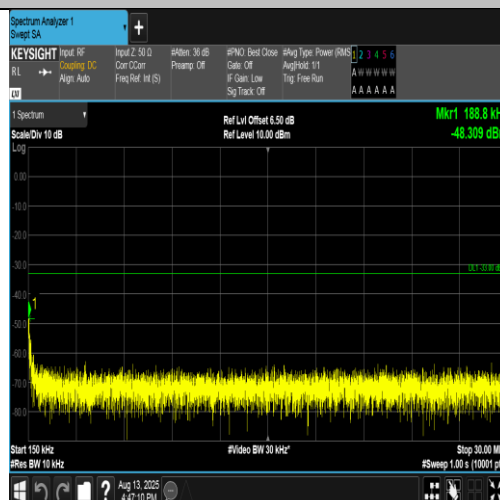
Band4-1513-4-0.15~30MHz-PASS
