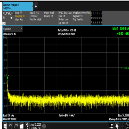
Band4-1513-1-0.15~30MHz-PASS
