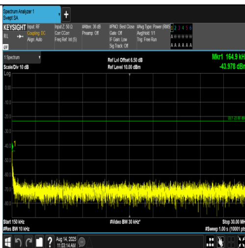
Band5-4233-4-0.15~30MHz-PASS
