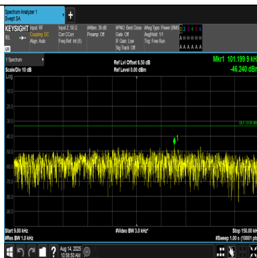
Band5-4233-2-0.009~0.15MHz-PASS
