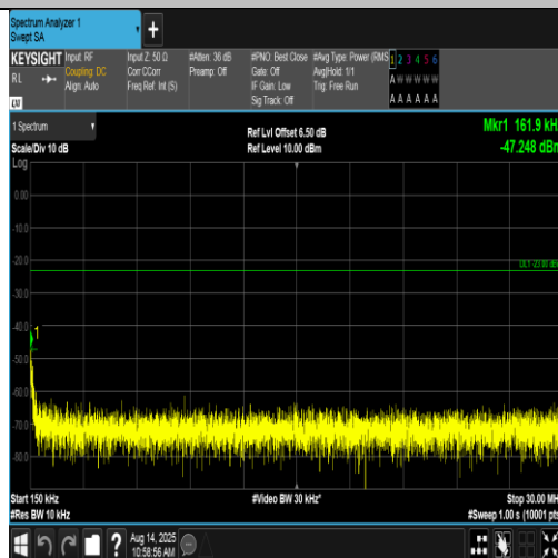
Band5-4233-2-0.15~30MHz-PASS
