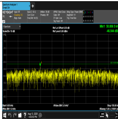
Band4-1413-3-0.009~0.15MHz-PASS
