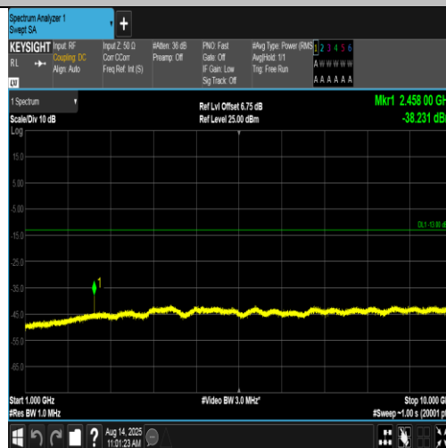
Band5-4233-3-1000~10000MHz-PASS
