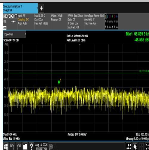
Band5-4233-4-0.009~0.15MHz-PASS
