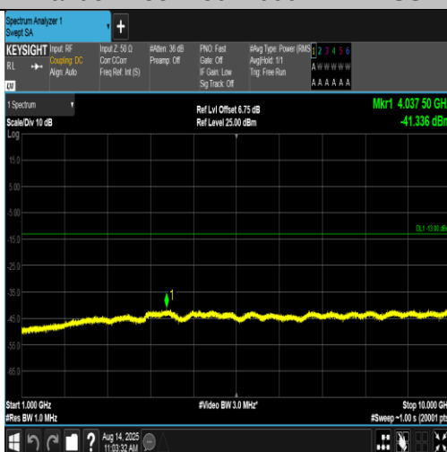
Band5-4233-4-1000~10000MHz-PASS
