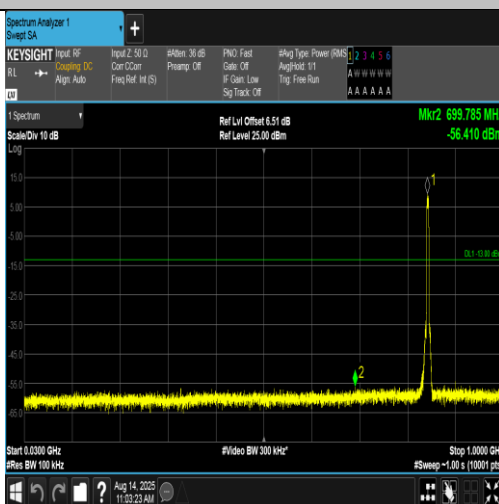
Band5-4233-4-30~1000MHz-PASS
