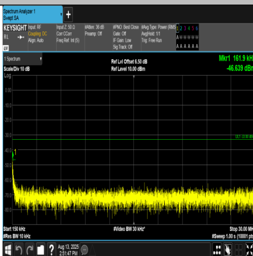
Band2-9262-1-0.15~30MHz-PASS
