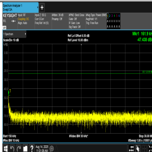
Band5-4233-3-0.15~30MHz-PASS
