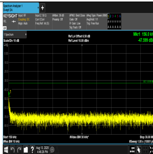
Band4-1413-4-0.15~30MHz-PASS
