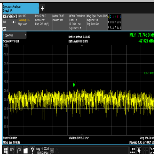
Band5-4233-1-0.009~0.15MHz-PASS
