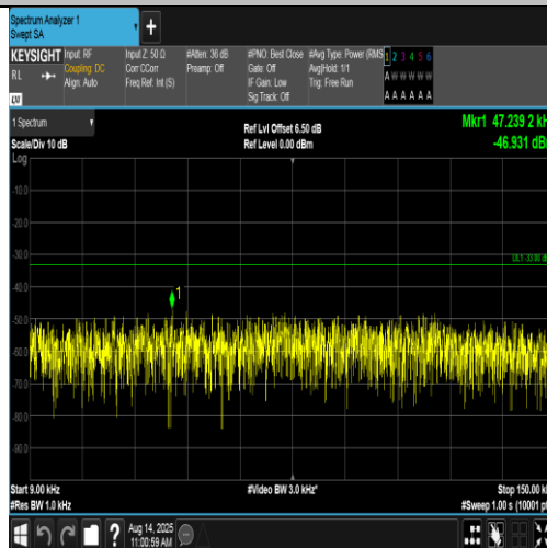
Band5-4233-3-0.009~0.15MHz-PASS
