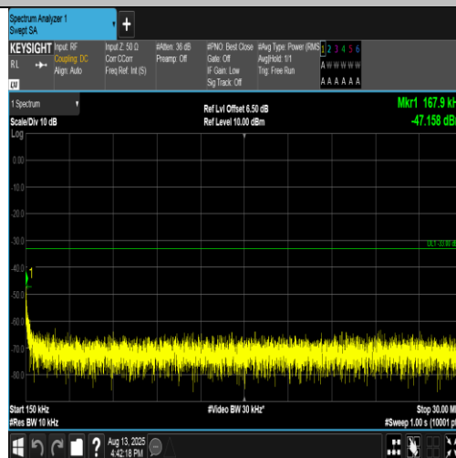
Band4-1513-2-0.15~30MHz-PASS
