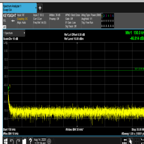
Band5-4182-4-0.15~30MHz-PASS
