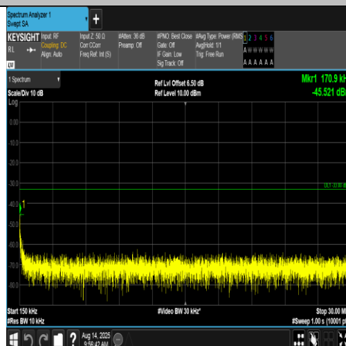
Band4-1513-2-0.15~30MHz-PASS
