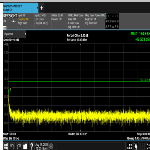
Band4-1513-3-0.15~30MHz-PASS
