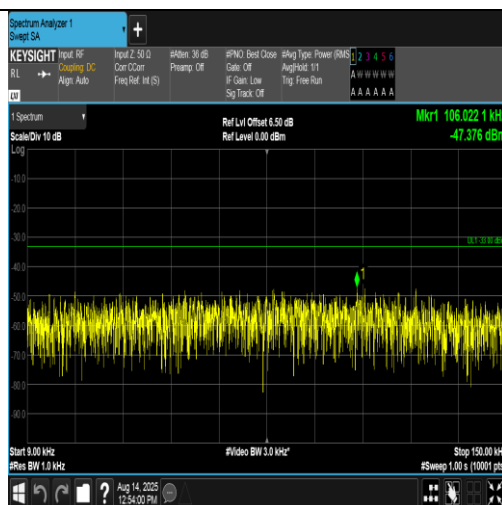
Band5-4132-4-0.009~0.15MHz-PASS
