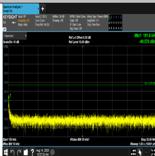
Band4-1413-5-0.15~30MHz-PASS
