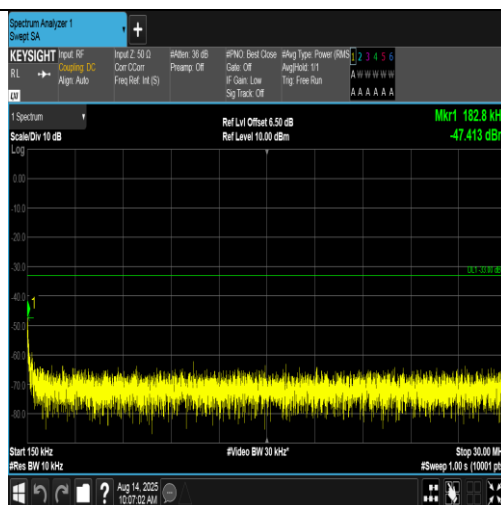
Band4-1312-5-0.15~30MHz-PASS
