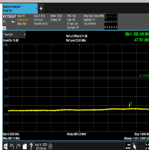
Band4-1513-1-30~1000MHz-PASS
