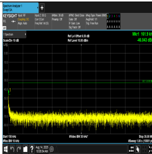
Band4-1513-4-0.15~30MHz-PASS
