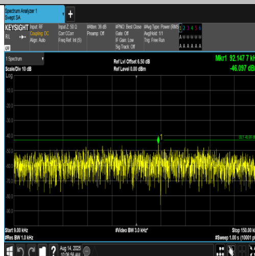
Band4-1312-5-0.009~0.15MHz-PASS
