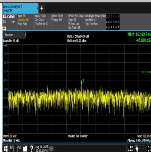
Band5-4182-1-0.009~0.15MHz-PASS
