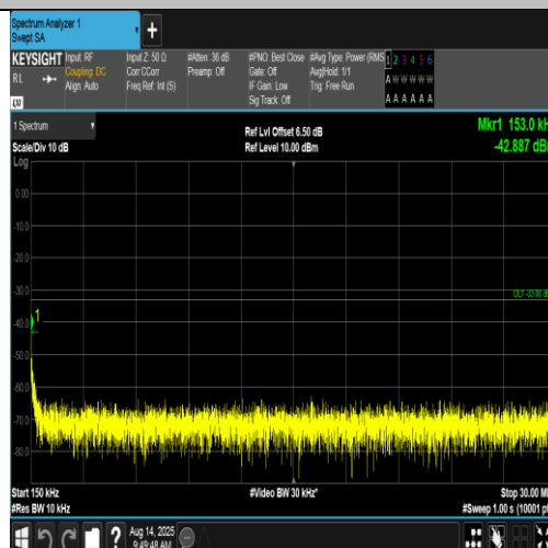
Band4-1413-1-0.15~30MHz-PASS
