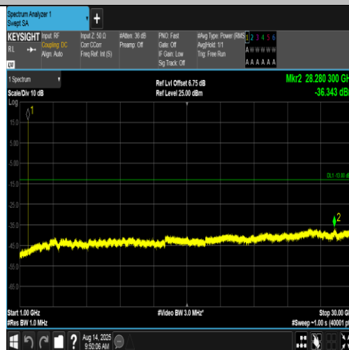
Band4-1413-1-1000~30000MHz-PASS
