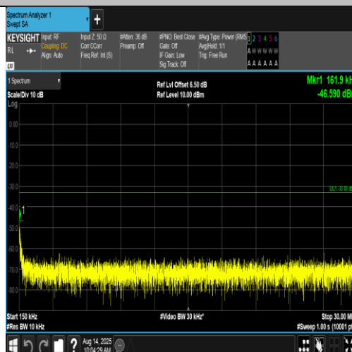
Band4-1413-4-0.15~30MHz-PASS
