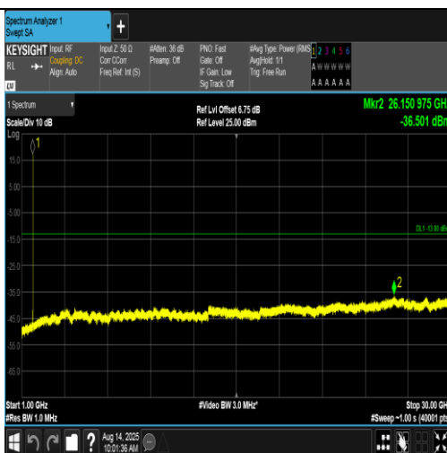
Band4-1513-3-1000~30000MHz-PASS
