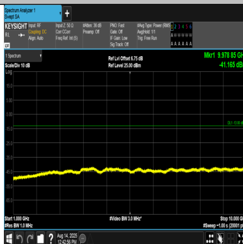
Band5-4182-1-1000~10000MHz-PASS
