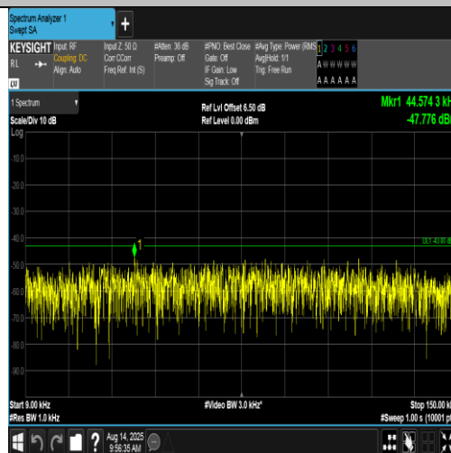
Band4-1513-2-0.009~0.15MHz-PASS
