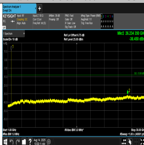
Band4-1413-3-1000~30000MHz-PASS
