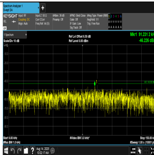
Band4-1312-4-0.009~0.15MHz-PASS
