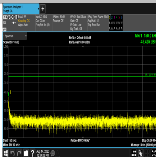
Band5-4132-4-0.15~30MHz-PASS
