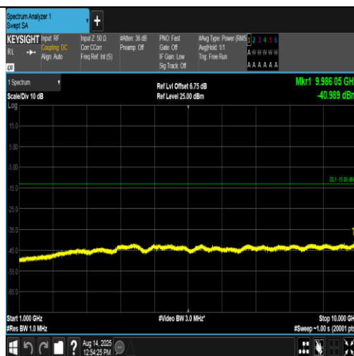
Band5-4132-4-1000~10000MHz-PASS
