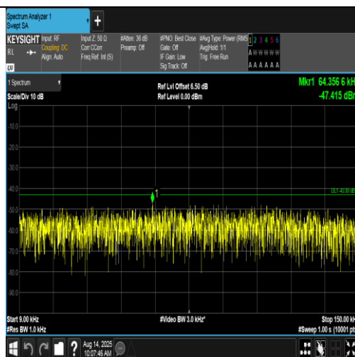
Band4-1413-5-0.009~0.15MHz-PASS
