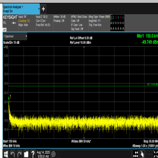
Band4-1413-2-0.15~30MHz-PASS
