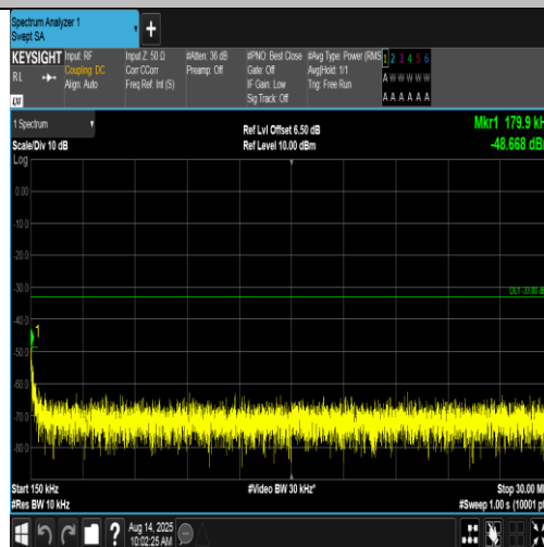
Band4-1312-4-0.15~30MHz-PASS
