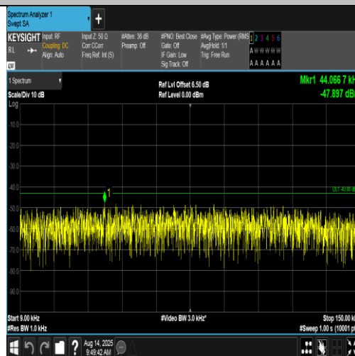
Band4-1413-1-0.009~0.15MHz-PASS
