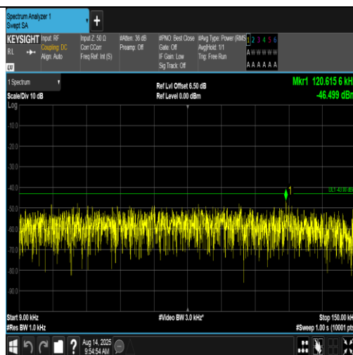
Band4-1413-2-0.009~0.15MHz-PASS
