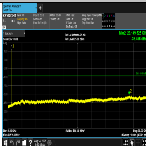
Band4-1513-1-1000~30000MHz-PASS
