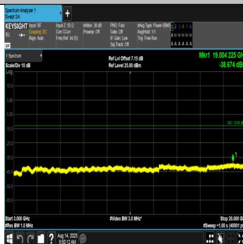
Band4-1413-1-3000~20000MHz-PASS
