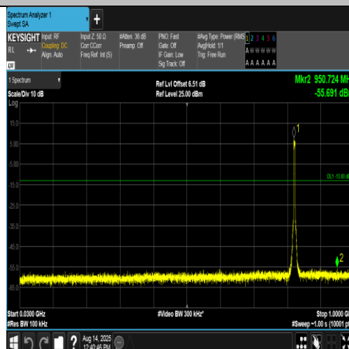
Band5-4132-1-30~1000MHz-PASS
