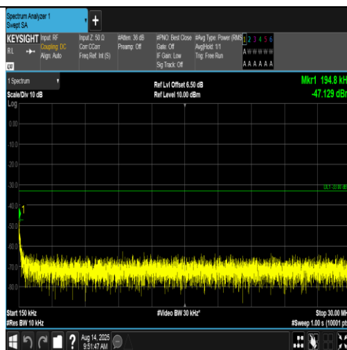
Band4-1513-1-0.15~30MHz-PASS
