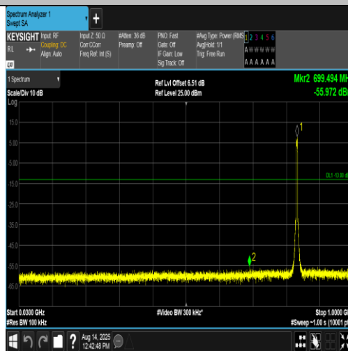
Band5-4182-1-30~1000MHz-PASS
