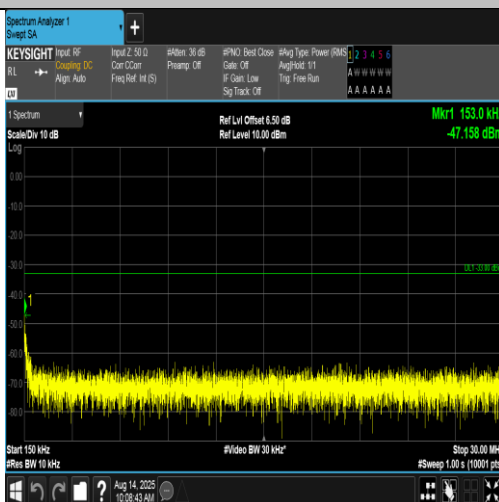
Band4-1513-5-0.15~30MHz-PASS
