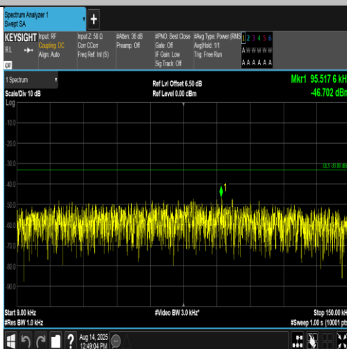
Band5-4132-3-0.009~0.15MHz-PASS
