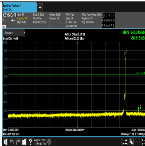
Band5-4132-5-30~1000MHz-PASS
