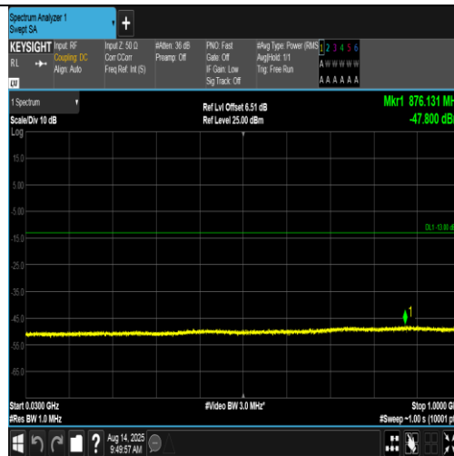
Band4-1413-1-30~1000MHz-PASS
