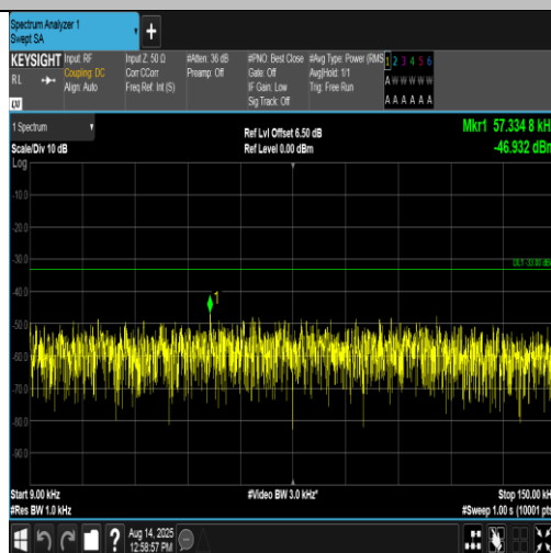
Band5-4132-5-0.009~0.15MHz-PASS
