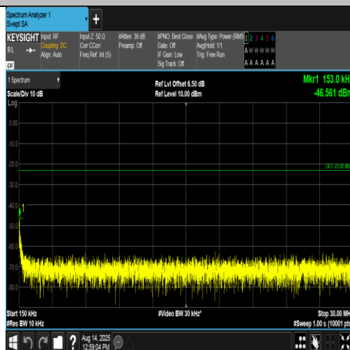
Band5-4132-5-0.15~30MHz-PASS
