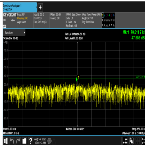
Band4-1513-3-0.009~0.15MHz-PASS
