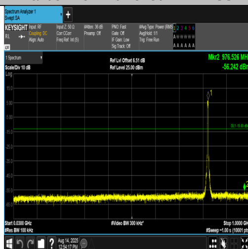
Band5-4132-4-30~1000MHz-PASS
