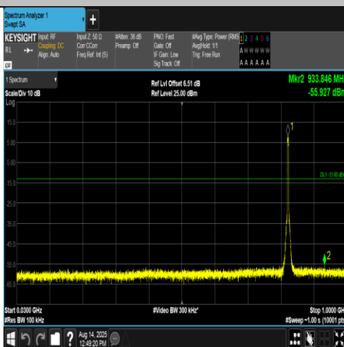
Band5-4132-3-30~1000MHz-PASS
