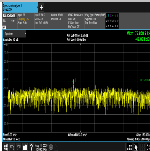
Band4-1413-4-0.009~0.15MHz-PASS
