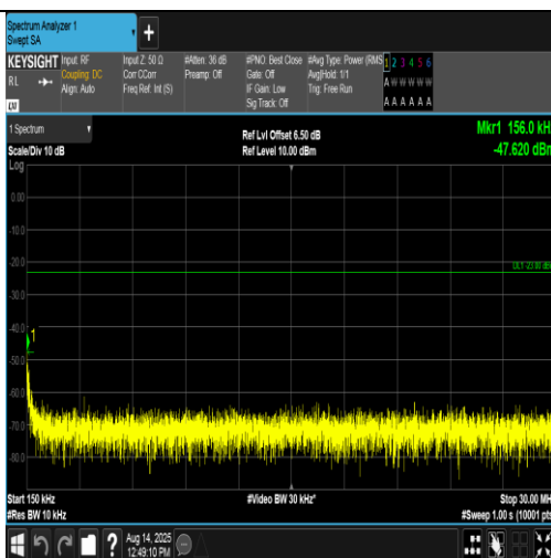
Band5-4132-3-0.15~30MHz-PASS
