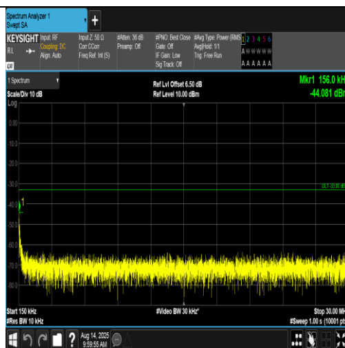
Band4-1413-3-0.15~30MHz-PASS
