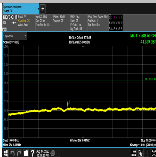
Band5-4182-3-1000~10000MHz-PASS
