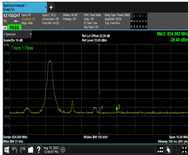
Band26-3MHz-16QAM-26775-1RB#14
