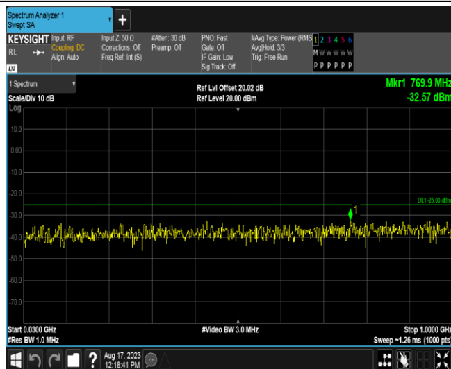
Band41-10MHz-16QAM-39700-1RB#0-Range1:30~1000MHz
