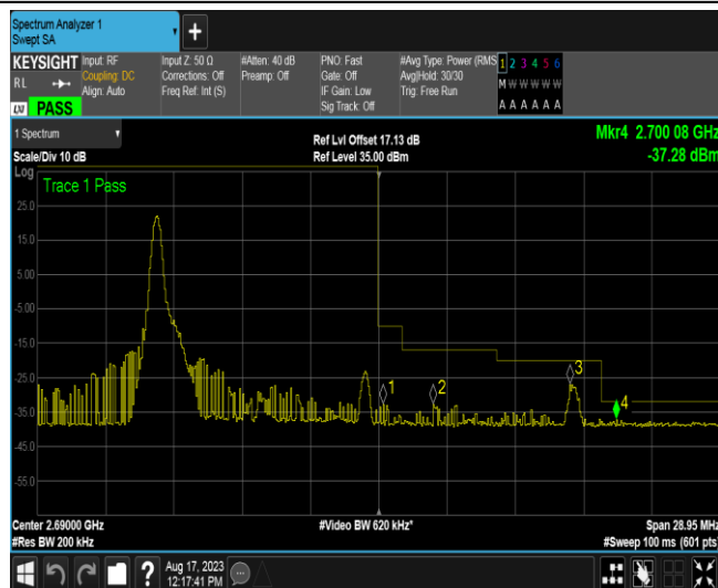
Band41-10MHz-16QAM-41540-1RB#0
