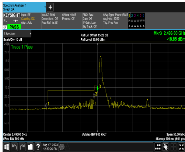
Band41-15MHz-QPSK-39725-1RB#74
