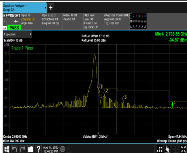
Band41-20MHz-QPSK-41490-100RB#0
