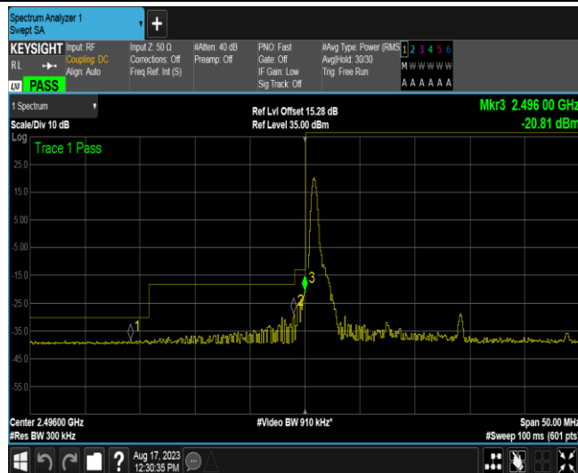
Band41-15MHz-16QAM-39725-1RB#74
