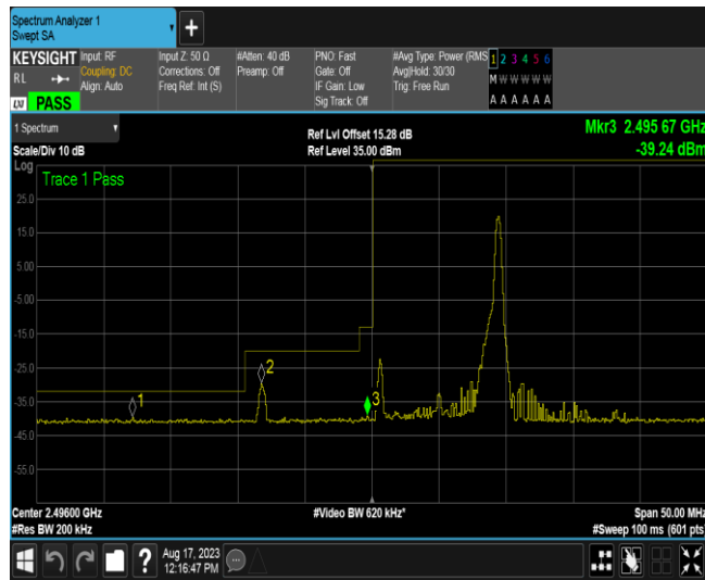
Band41-10MHz-16QAM-39700-50RB#0
