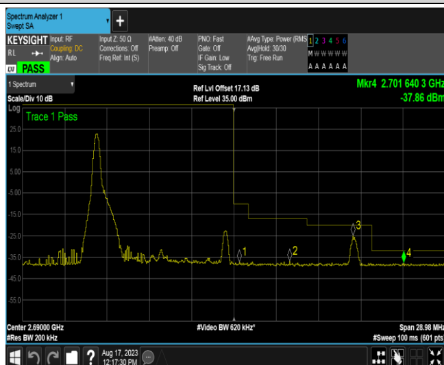
Band41-10MHz-QPSK-41540-1RB#49
