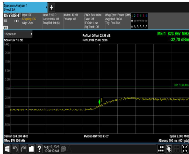
Band5-5MHz-16QAM-20425-25RB#0
