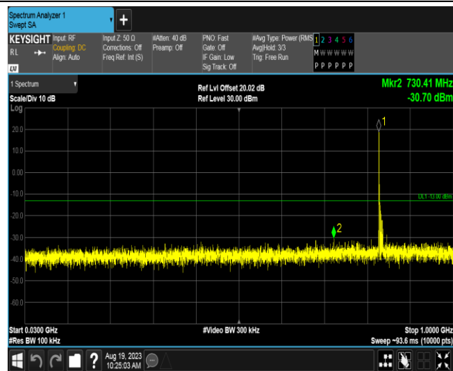
Band5-10MHz-QPSK-20525-1RB#0-Range1:30~1000MHz
