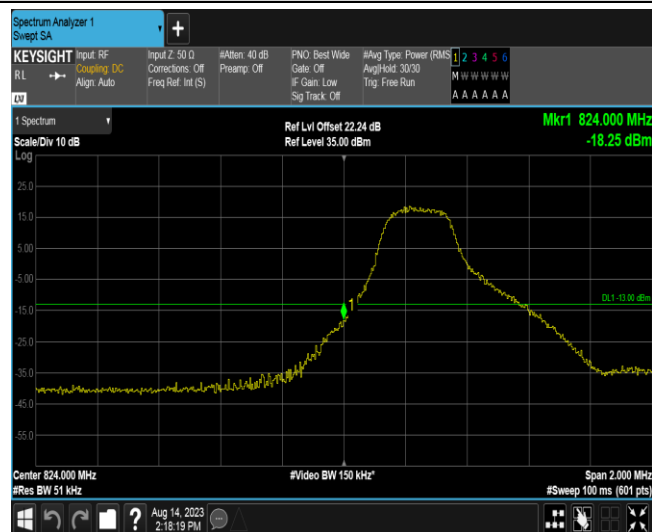
Band5-3MHz-16QAM-20415-1RB#0
