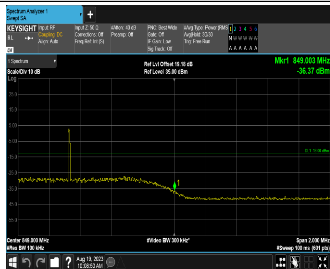
Band5-5MHz-16QAM-20625-1RB#0
