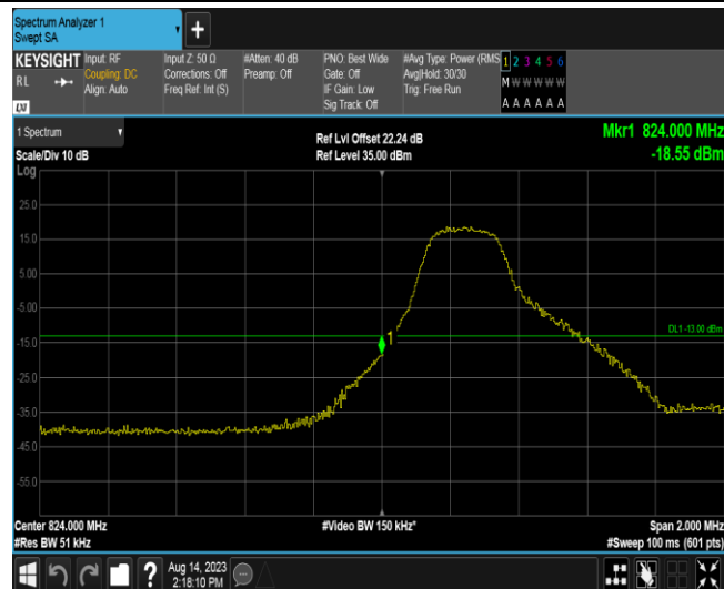
Band5-3MHz-QPSK-20415-1RB#14
