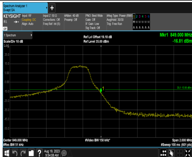
Band5-3MHz-16QAM-20635-15RB#0
