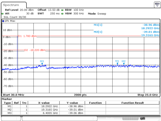
BLE_2M_Middle_Channel
