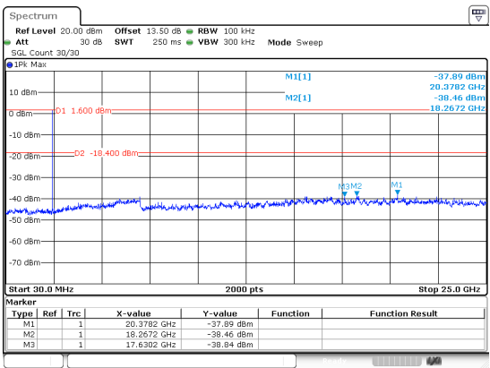
BLE_1M_Middle_Channel
