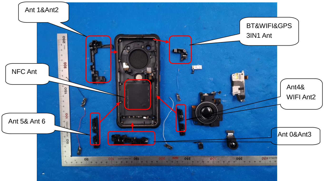
OPEN VIEW OF EUT(FIGURE 4)
