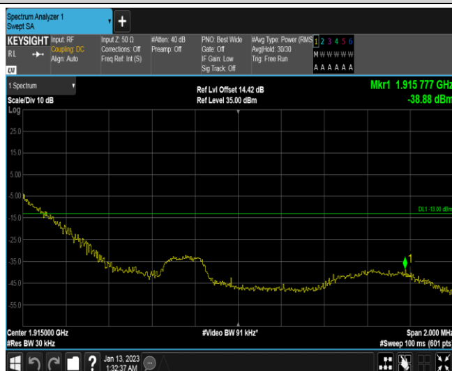
Band25-1.4MHz-QPSK-26683-1RB#5
