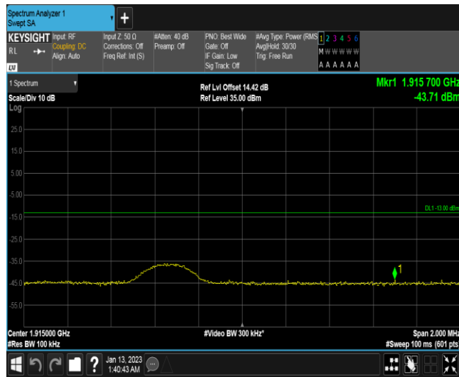
Band25-5MHz-QPSK-26665-1RB#24
