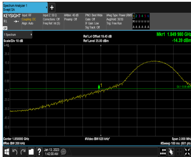
Band25-10MHz-16QAM-26090-1RB#49
