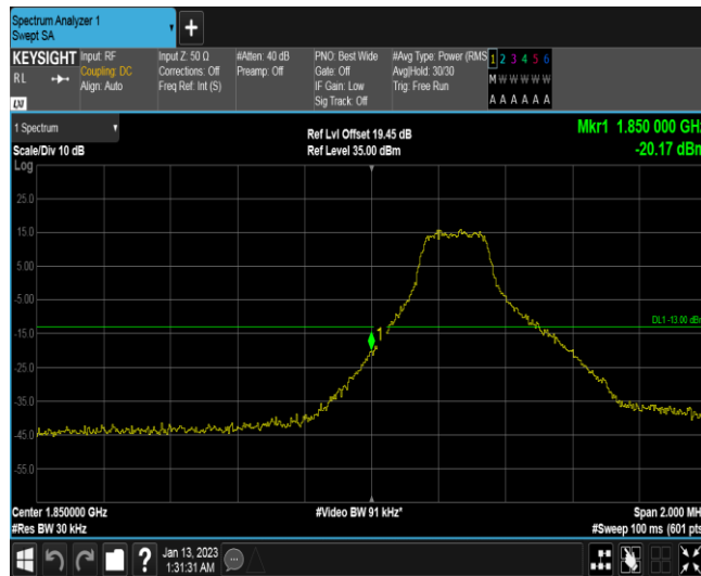
Band25-1.4MHz-QPSK-26047-1RB#5
