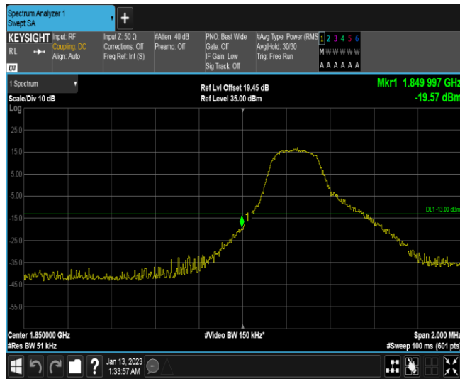
Band25-3MHz-QPSK-26055-1RB#14
