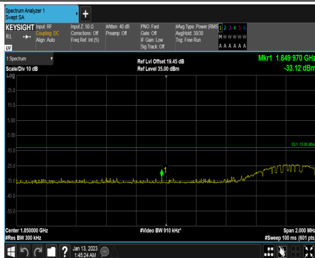
Band25-15MHz-QPSK-26115-1RB#74
