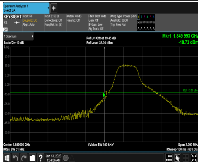
Band25-3MHz-16QAM-26055-1RB#14
