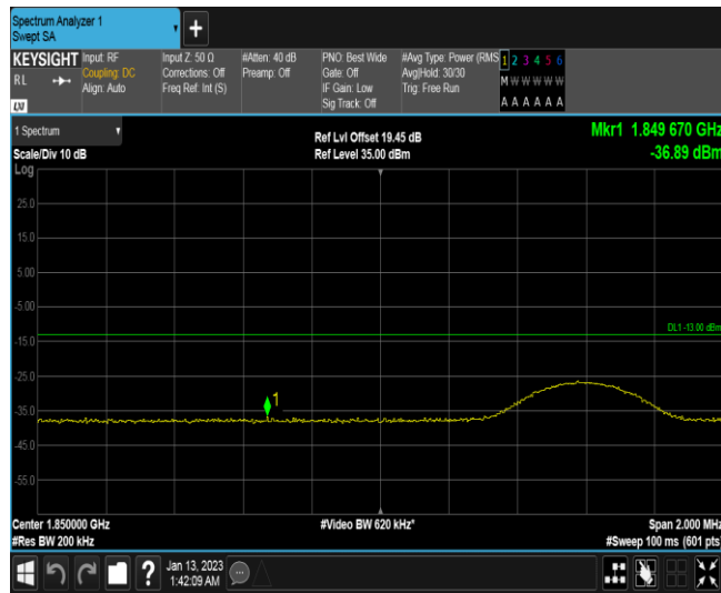
Band25-10MHz-QPSK-26090-50RB#0
