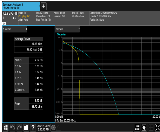
Band41-20MHz-QPSK-39750-100RB#0
