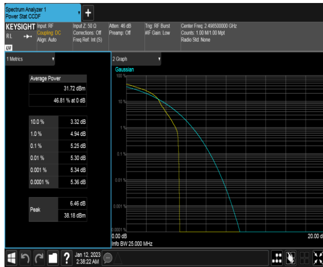
Band41-5MHz-16QAM-39675-25RB#0
