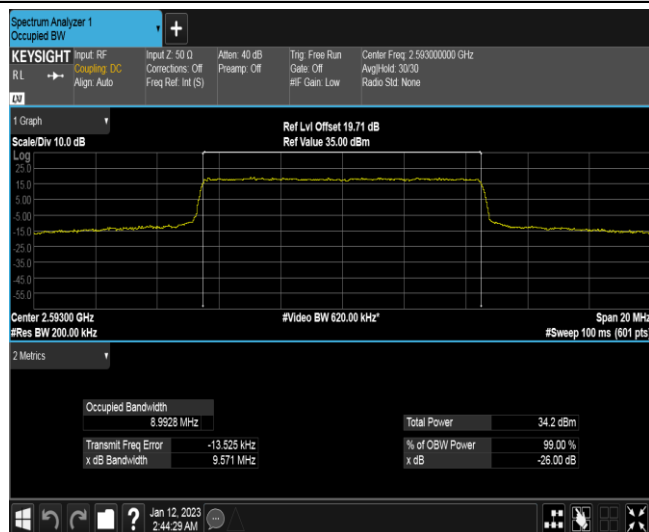
Band41-10MHz-QPSK-40620-50RB#0
