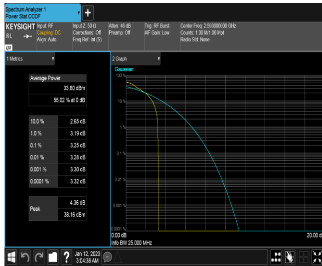
Band41-15MHz-QPSK-40620-75RB#0
