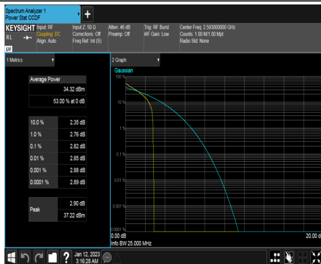
Band41-20MHz-QPSK-40620-1RB#0
