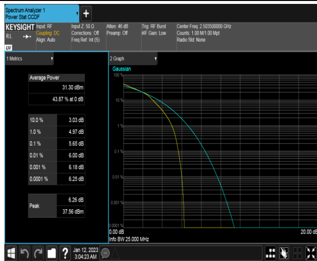
Band41-15MHz-16QAM-40620-1RB#0
