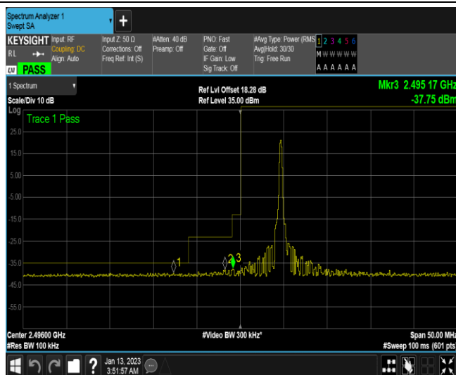
Band41-5MHz-QPSK-39675-25RB#0
