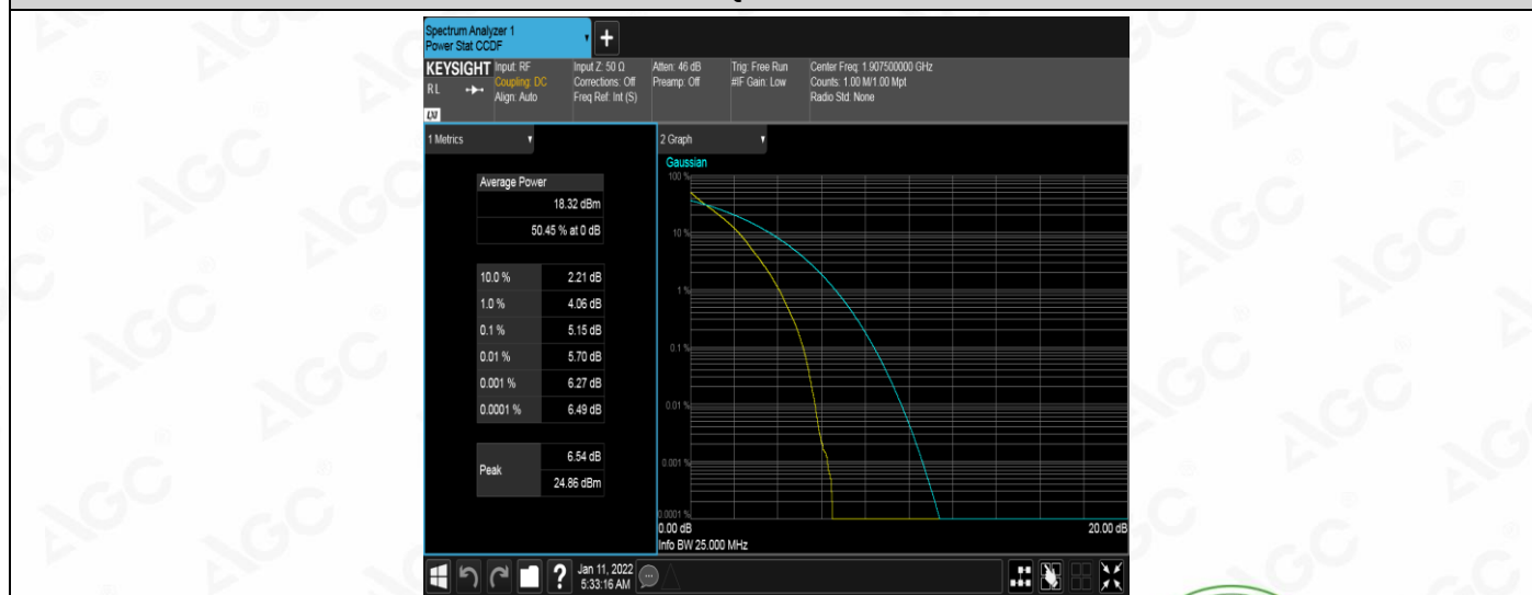
Band2-5MHz-QPSK-19175-25RB#0
