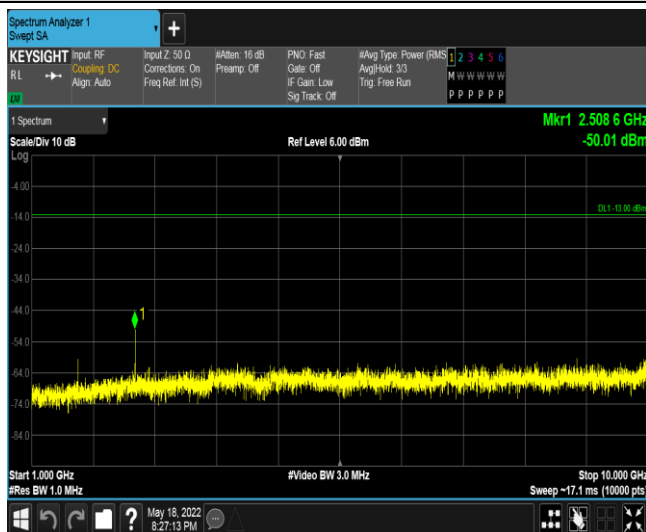
Band5-1.4MHz-16QAM-20525-1RB#0-Range3:1000~10000MHz
