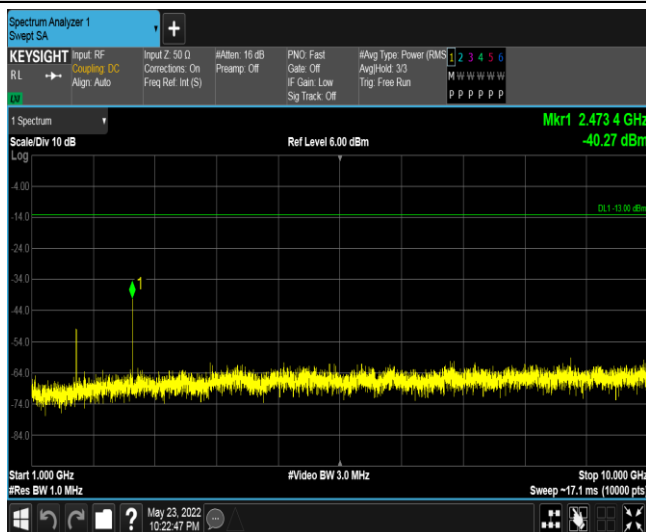
Band5-3MHz-16QAM-20415-1RB#0-Range3:1000~10000MHz
