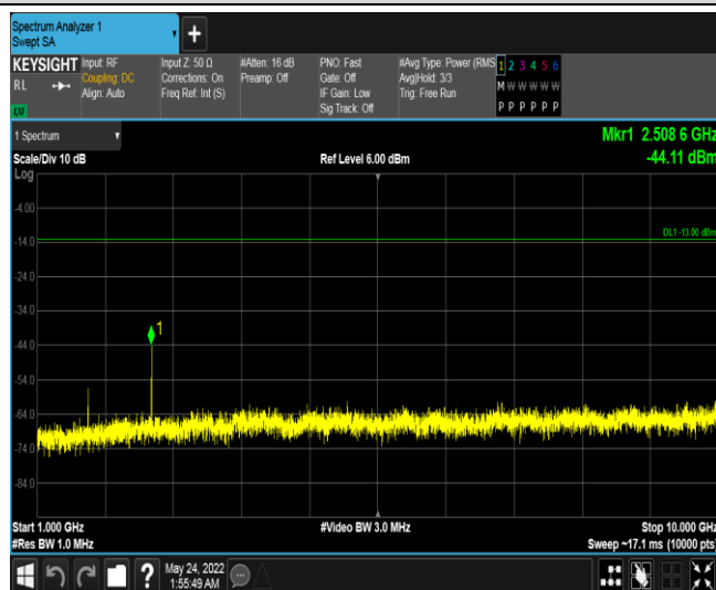
Band26-1.4MHz-QPSK-26915-1RB#0-Range3:1000~10000MHz
