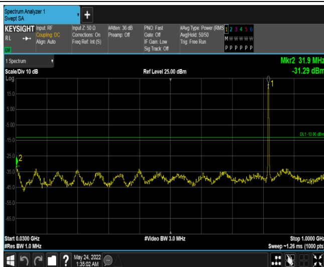
Band26-3MHz-QPSK-26775-1RB#0-Range2:30~1000MHz
