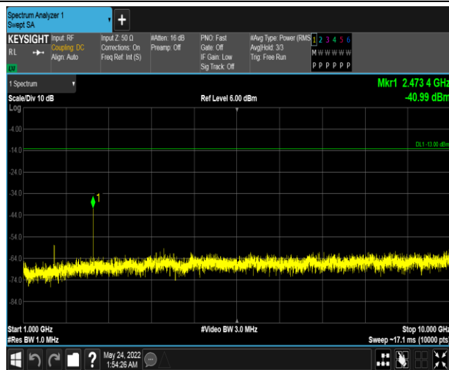
Band26-1.4MHz-16QAM-26797-1RB#0-Range3:1000~10000MHz
