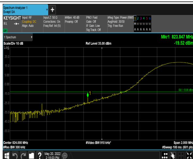
Band26-15MHz-QPSK-26865-1RB#74
