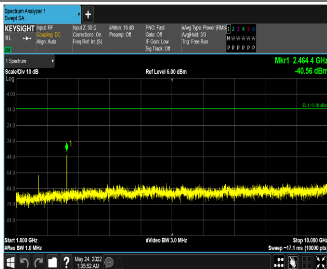
Band26-3MHz-QPSK-26775-1RB#0-Range3:1000~10000MHz
