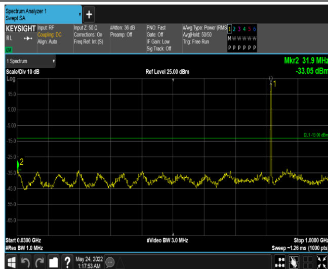
Band26-1.4MHz-QPSK-26740-1RB#0-Range2:30~1000MHz
