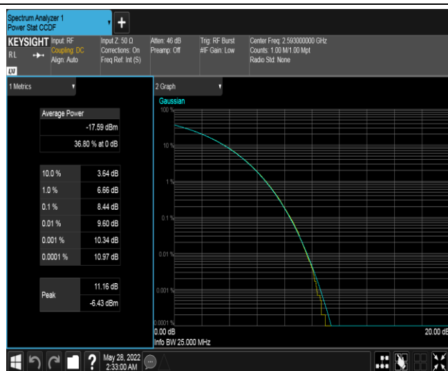
Band41-15MHz-QPSK-41515-1RB#0
