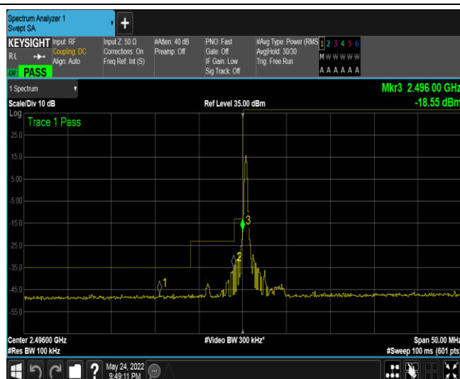
Band41-5MHz-16QAM-39675-1RB#24
