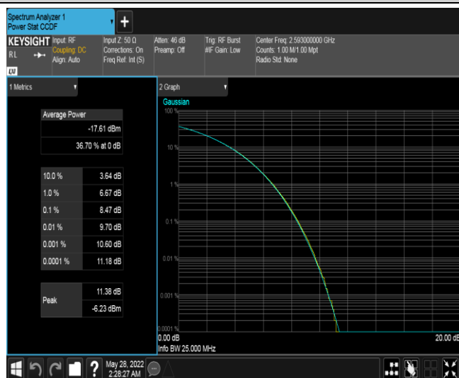
Band41-10MHz-QPSK-40620-1RB#0
