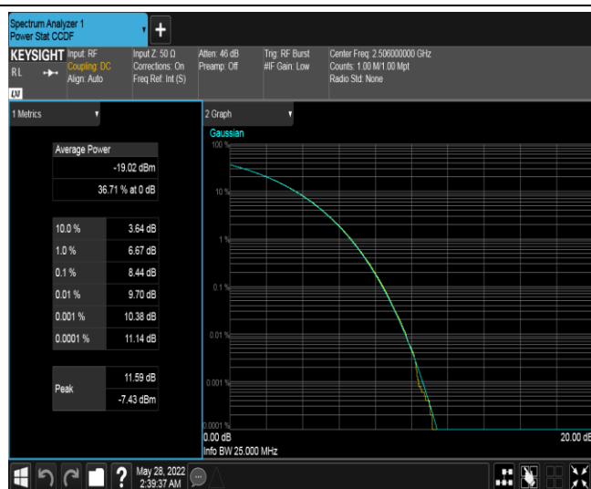
Band41-20MHz-QPSK-40620-1RB#0
