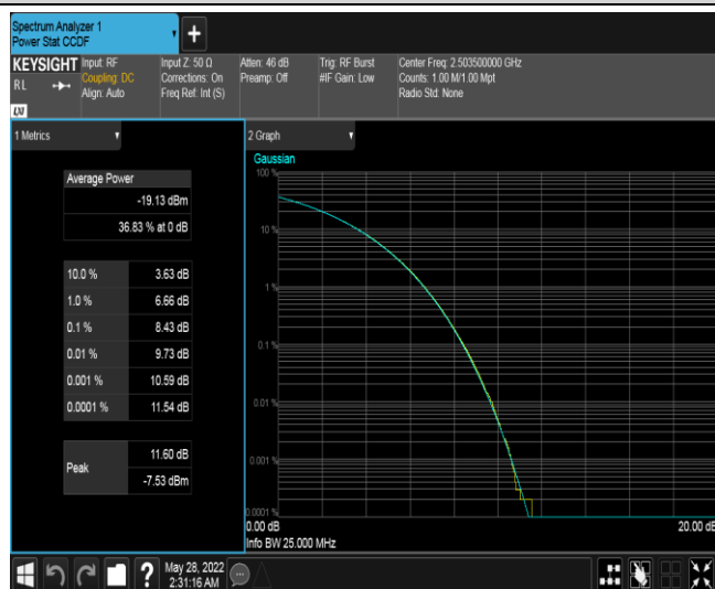
Band41-15MHz-QPSK-39725-1RB#0
