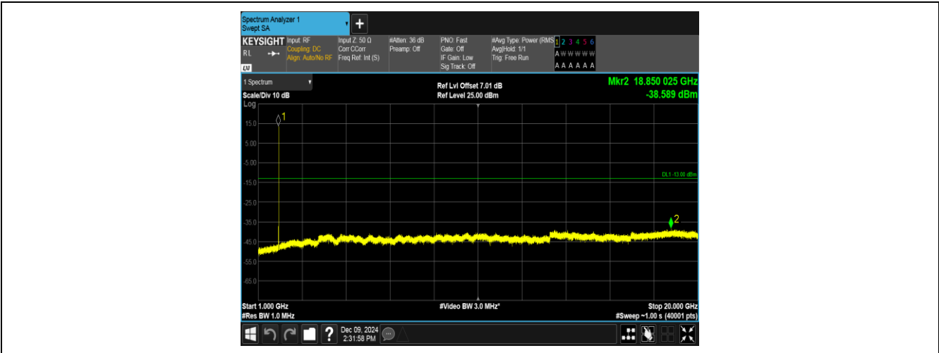
Band2-9400-2-1000~20000MHz-PASS
