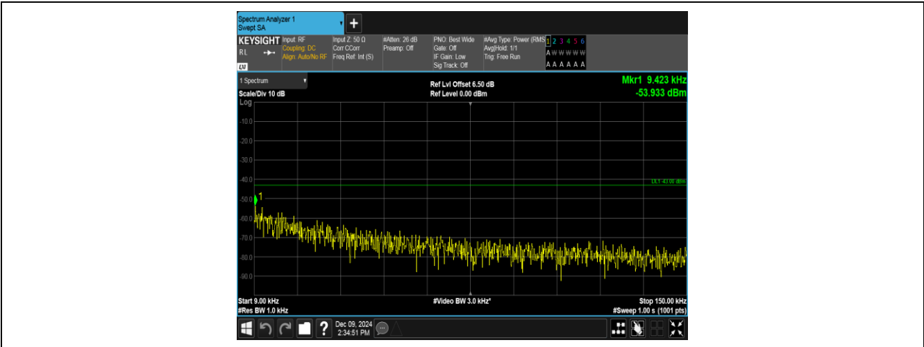
Band2-9538-3-0.009~0.15MHz-PASS
