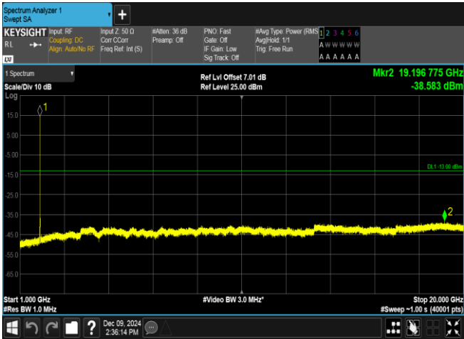
Band2-9262-4-1000~20000MHz-PASS
