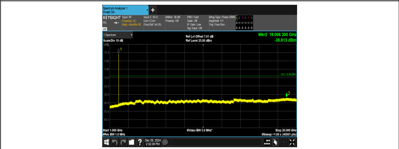
Band2-9538-2-1000~20000MHz-PASS
