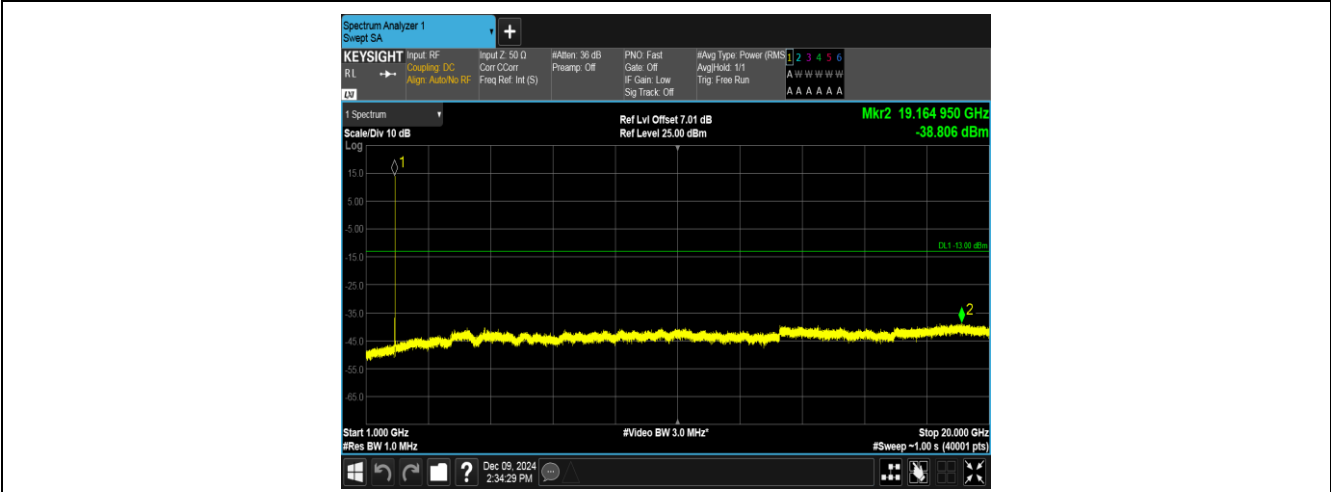
Band2-9400-3-1000~20000MHz-PASS
