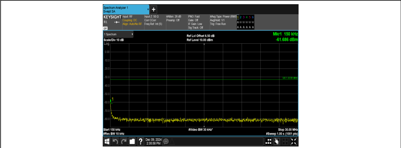
Band2-9262-4-0.15~30MHz-PASS
