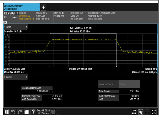
Band66-3MHz-16QAM-132657-15RB#0-PASS
