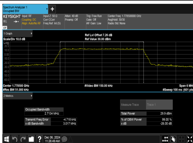
Band66-3MHz-QPSK-132657-15RB#0-PASS
