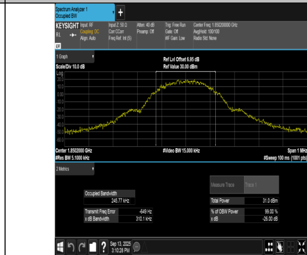
EGPRS1900-512-2-PASS
