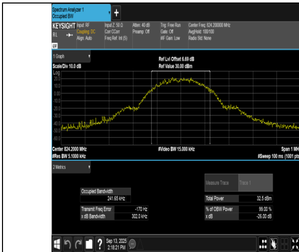
EGPRS850-128-8-PASS
