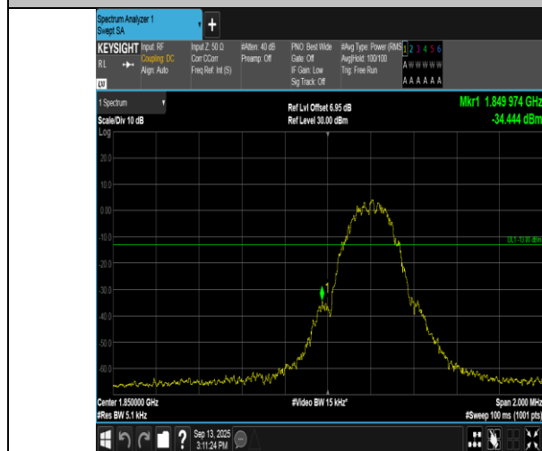
EGPRS1900-512-2-PASS
