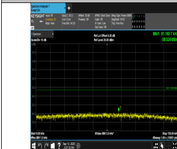
GPRS850-190-5-0.009~0.15MHz-PASS
